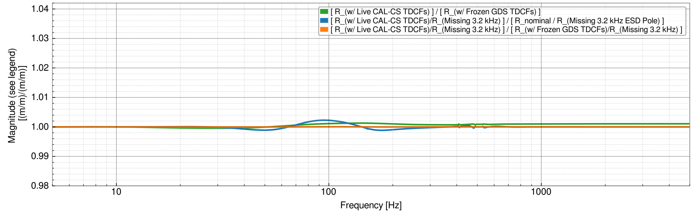
Systematic Error Comparison: Ratio of R_(w/ CALCS TDCFs) / R_(w/ GDS TDCFs) with and without Missing 3.2 kHz ESD Pole LHO:71787; THERMALIZED
