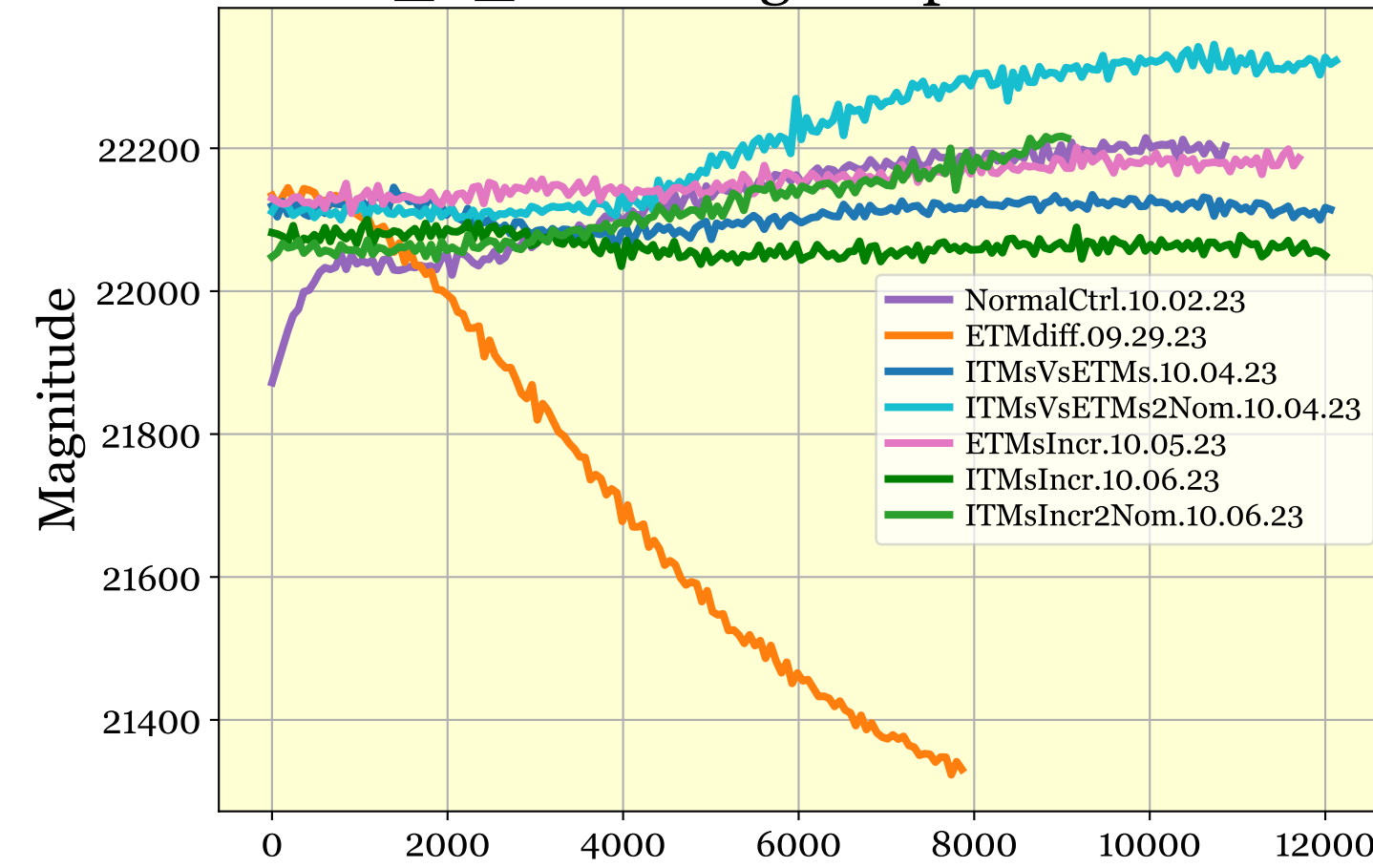
AS_A_RF45 mag and phase vs time
