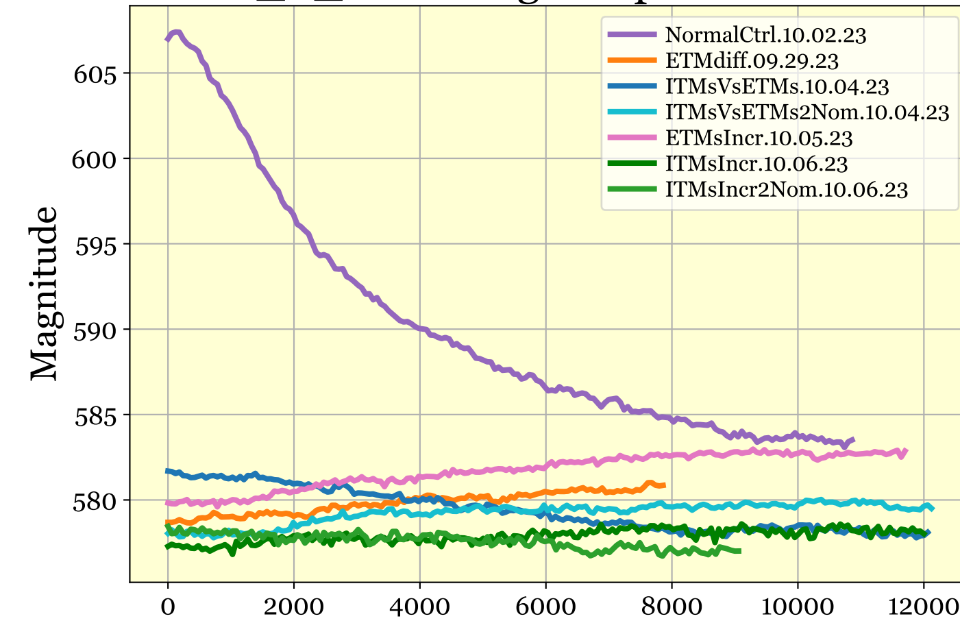
AS_A_RF72 mag and phase vs time
