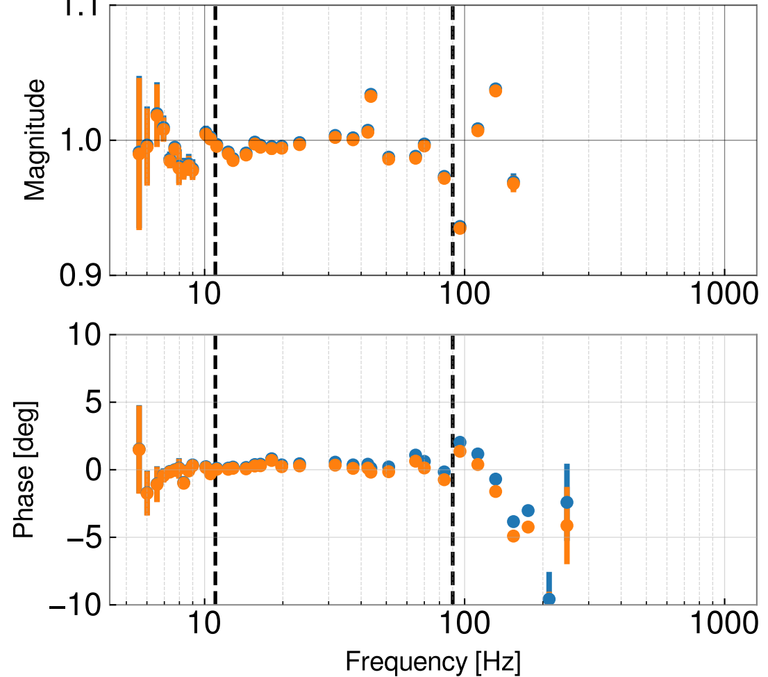
Actuation strength residuals (measurement/model w. free params)
