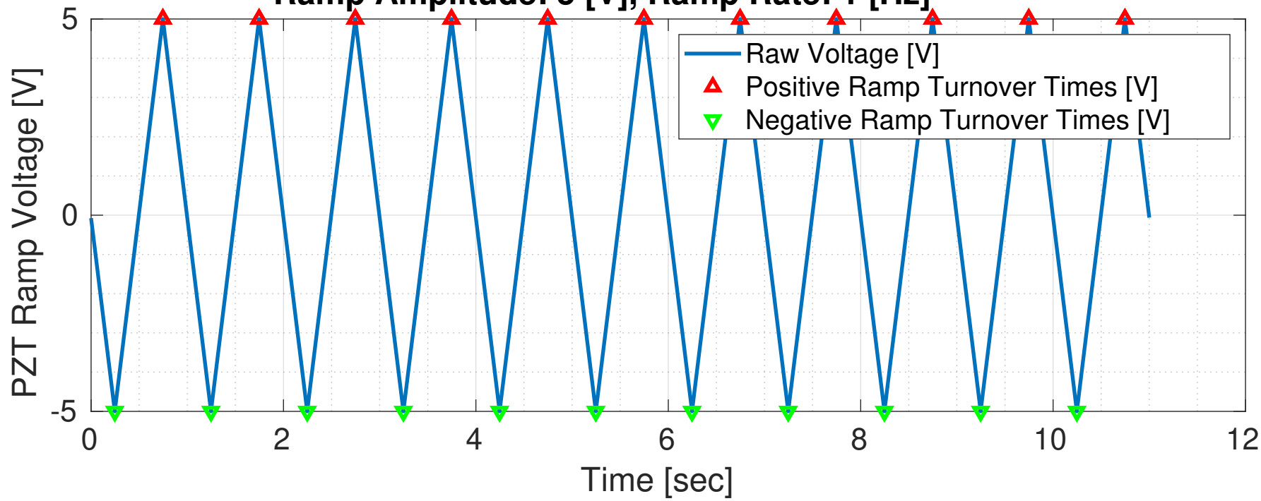
Ramp Amplitude: 5 [V], Ramp Rate: 1 [Hz]
