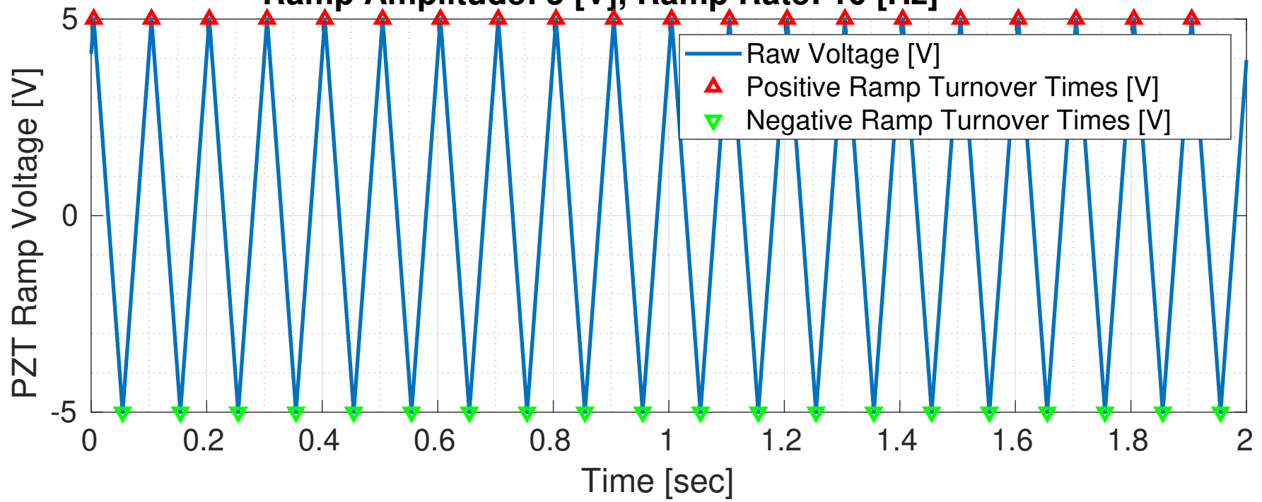
Ramp Amplitude: 5 [V], Ramp Rate: 10 [Hz]
