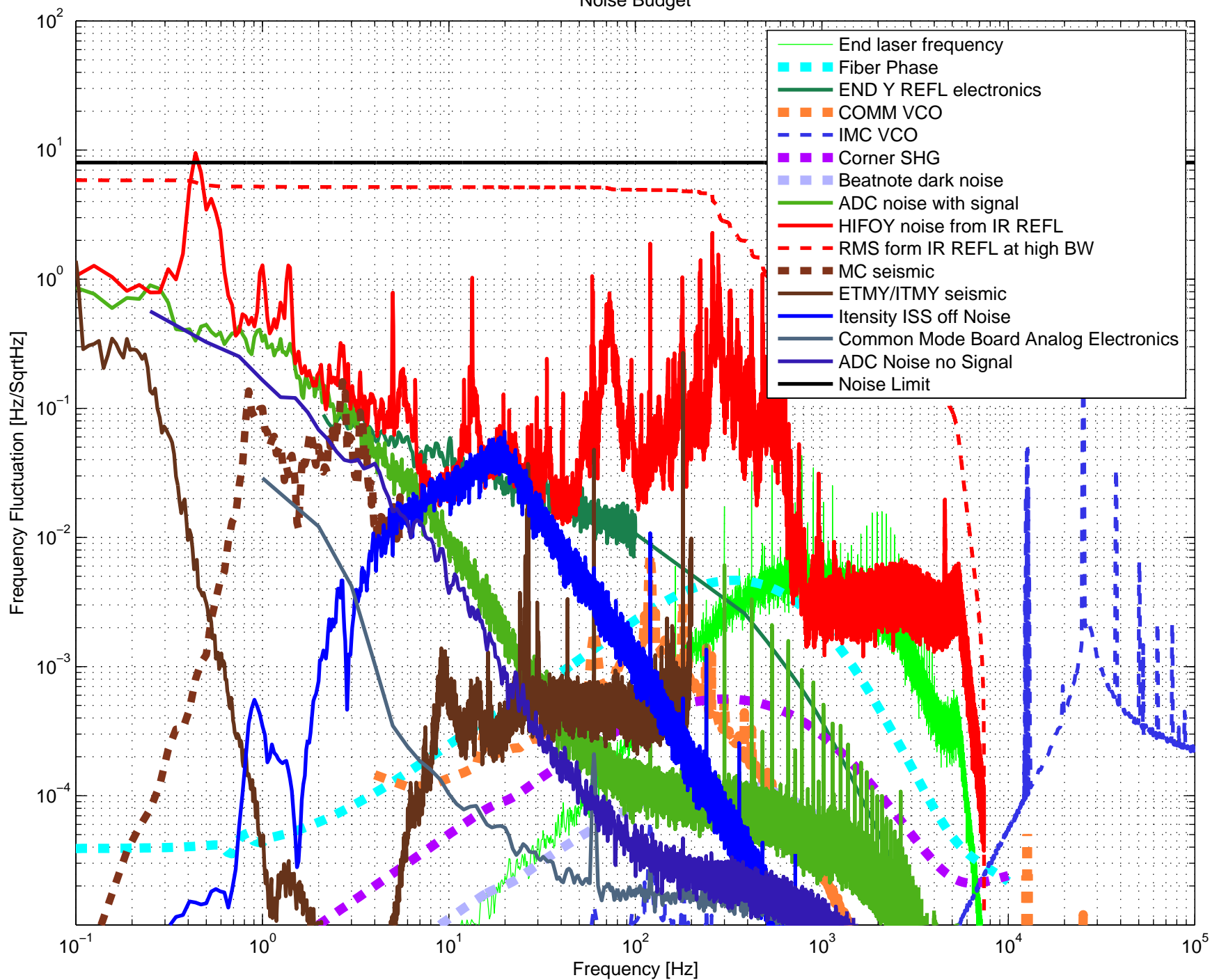
Noise Budget
