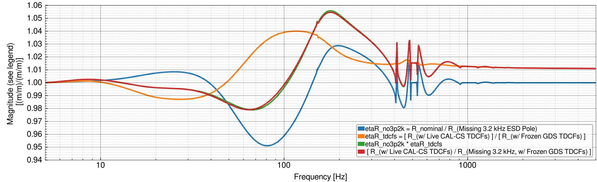
Systematic Error Comparison: Treating TDCF Update and No 3.2 kHz Pole as Separable Independent vs "The right thing" LHO:72622; NOT THERMALIZED
