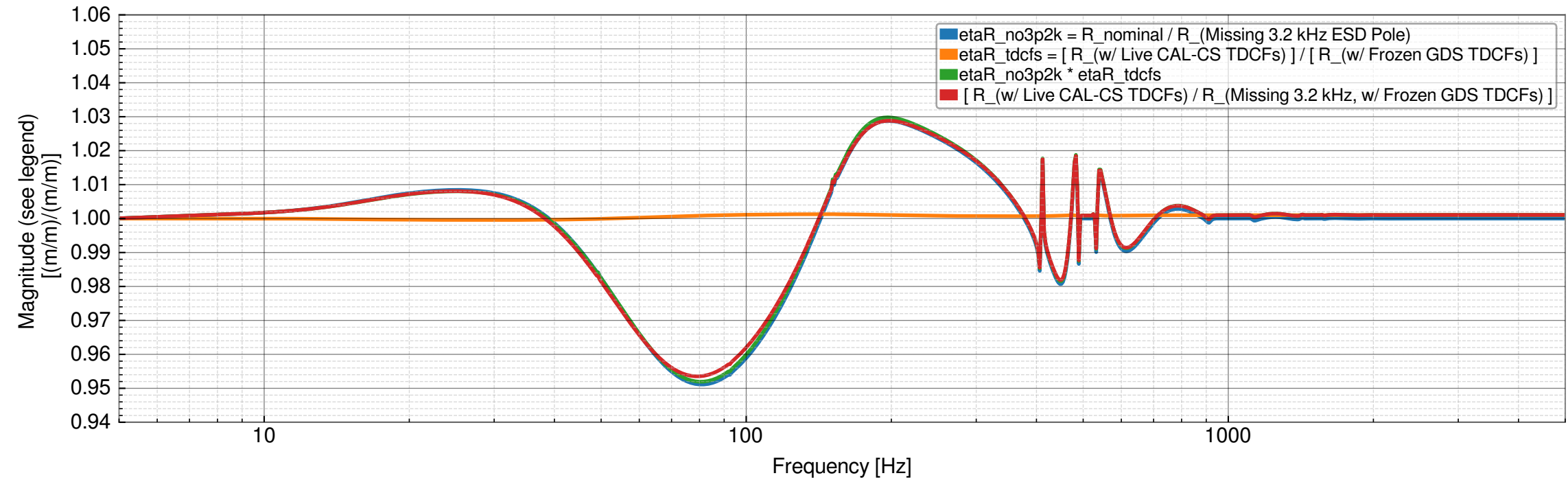
Systematic Error Comparison: Treating TDCF Update and No 3.2 kHz Pole as Separable Independent vs "The right thing" LHO:71787; THERMALIZED
