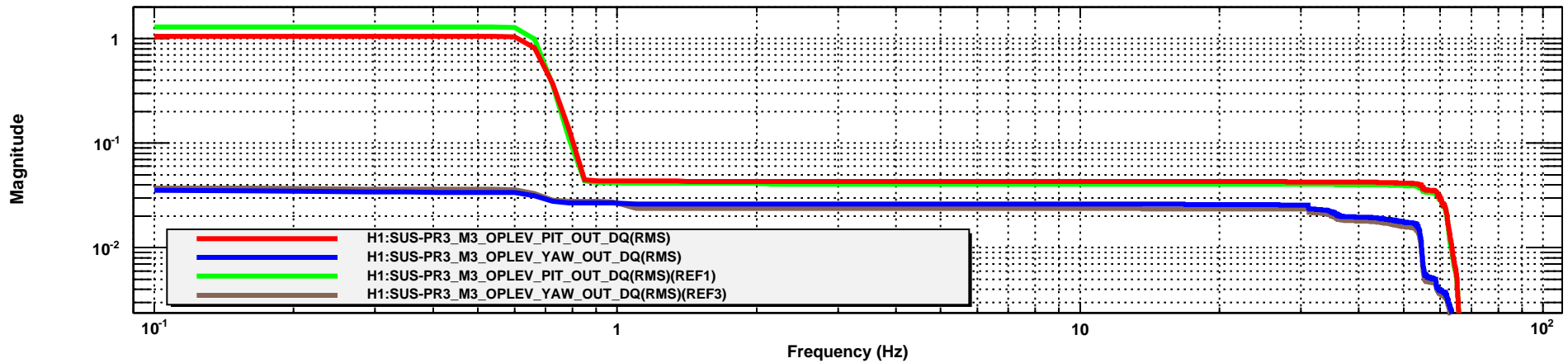
Power spectrum
