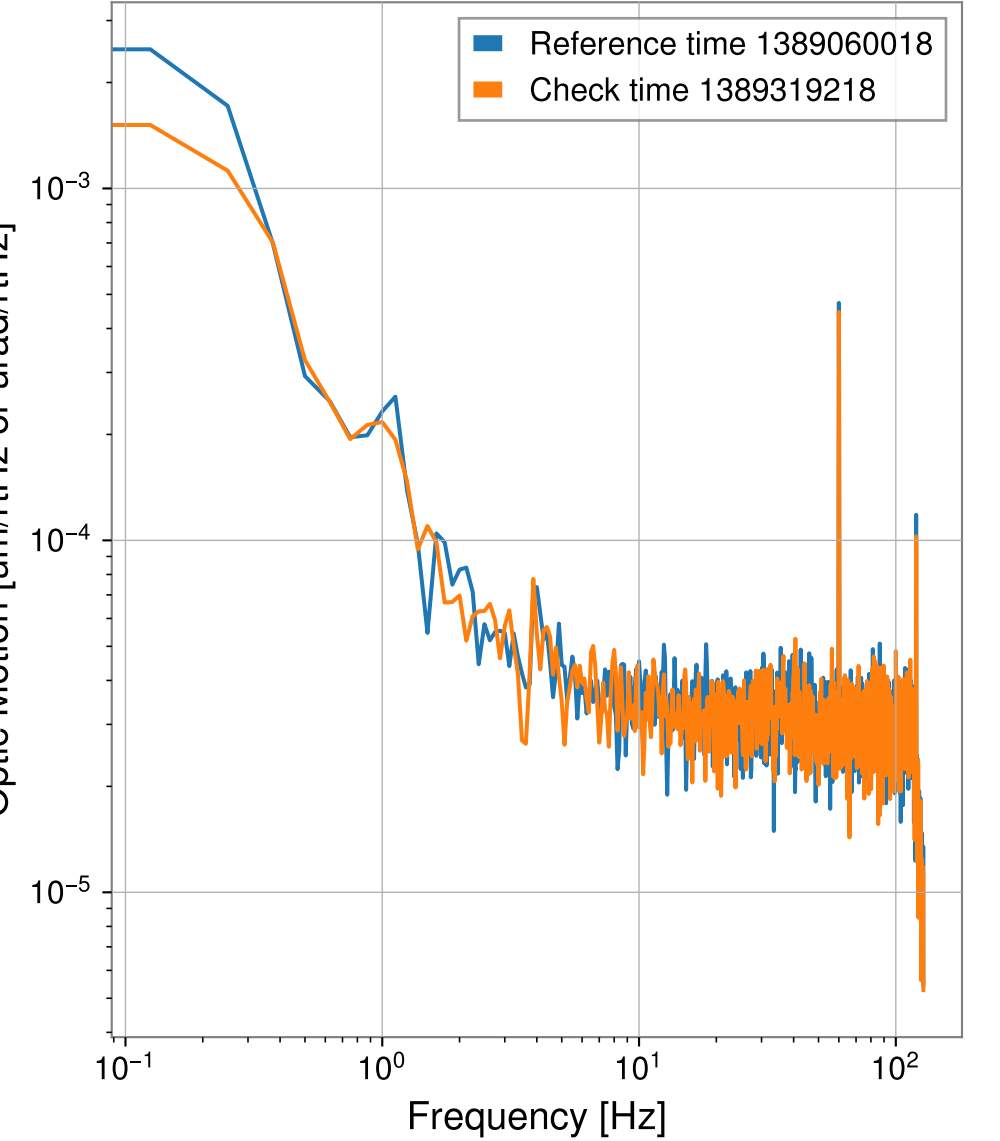
H1:SUS-BS_M1_DAMP_V_IN1_DQ
