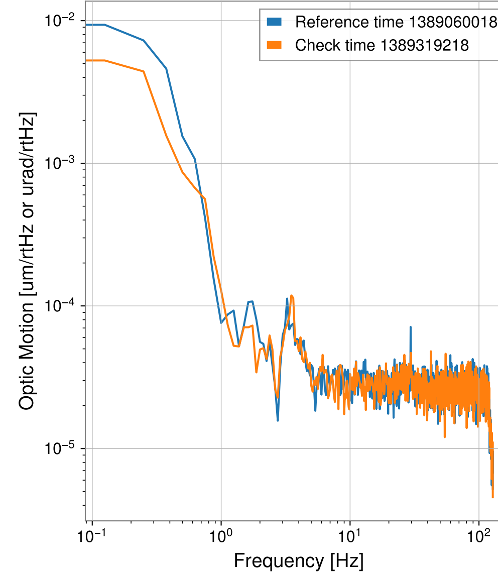
H1:SUS-MC3_M1_DAMP_L_IN1_DQ
