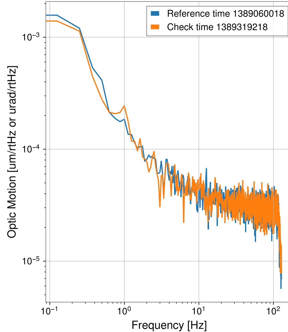
H1:SUS-SR3_M1_DAMP_V_IN1_DQ
