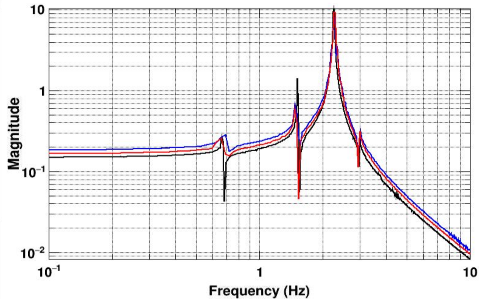
Transfer function
