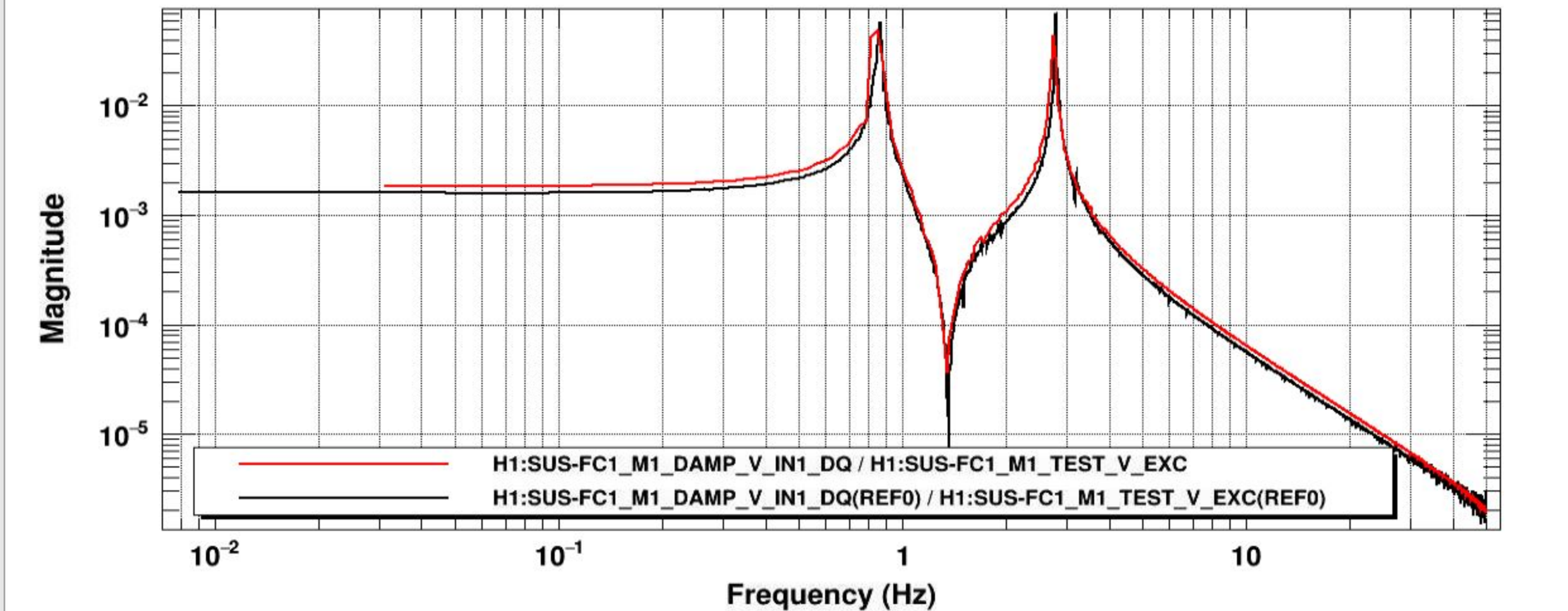
Transfer function
