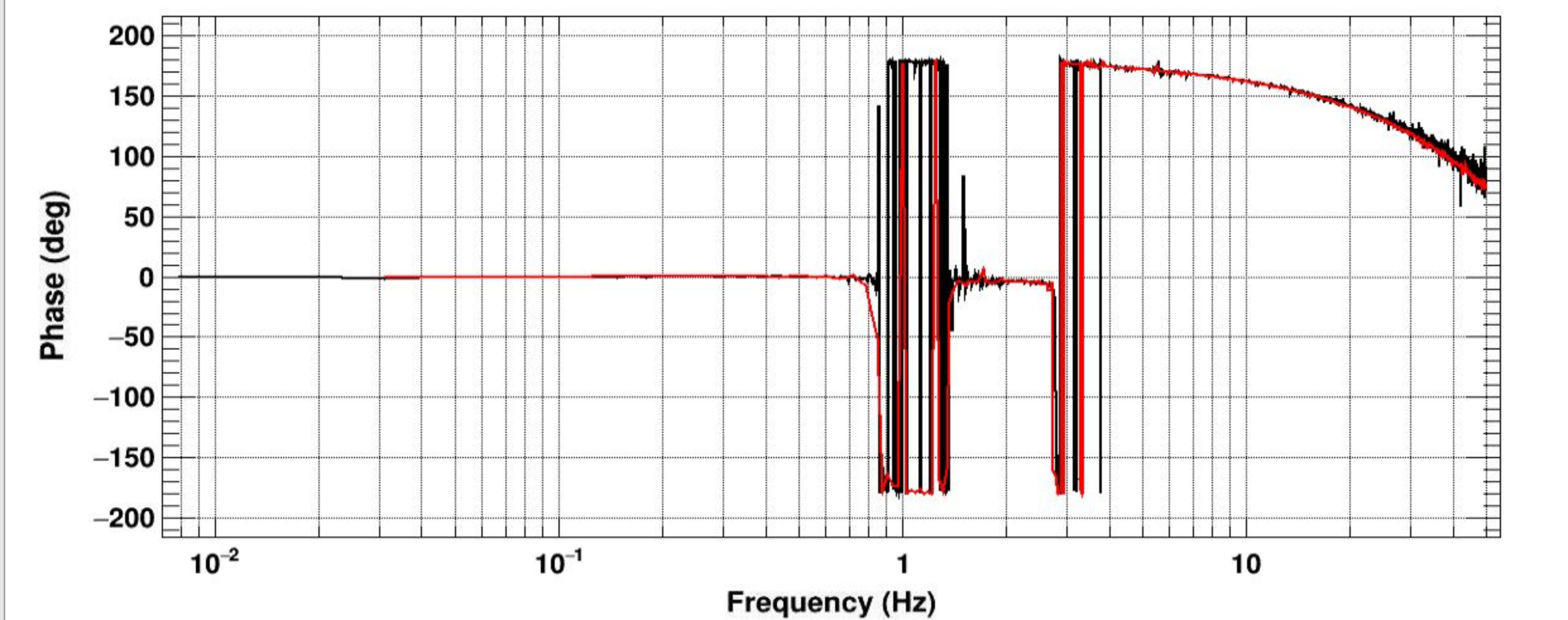
Transfer function
