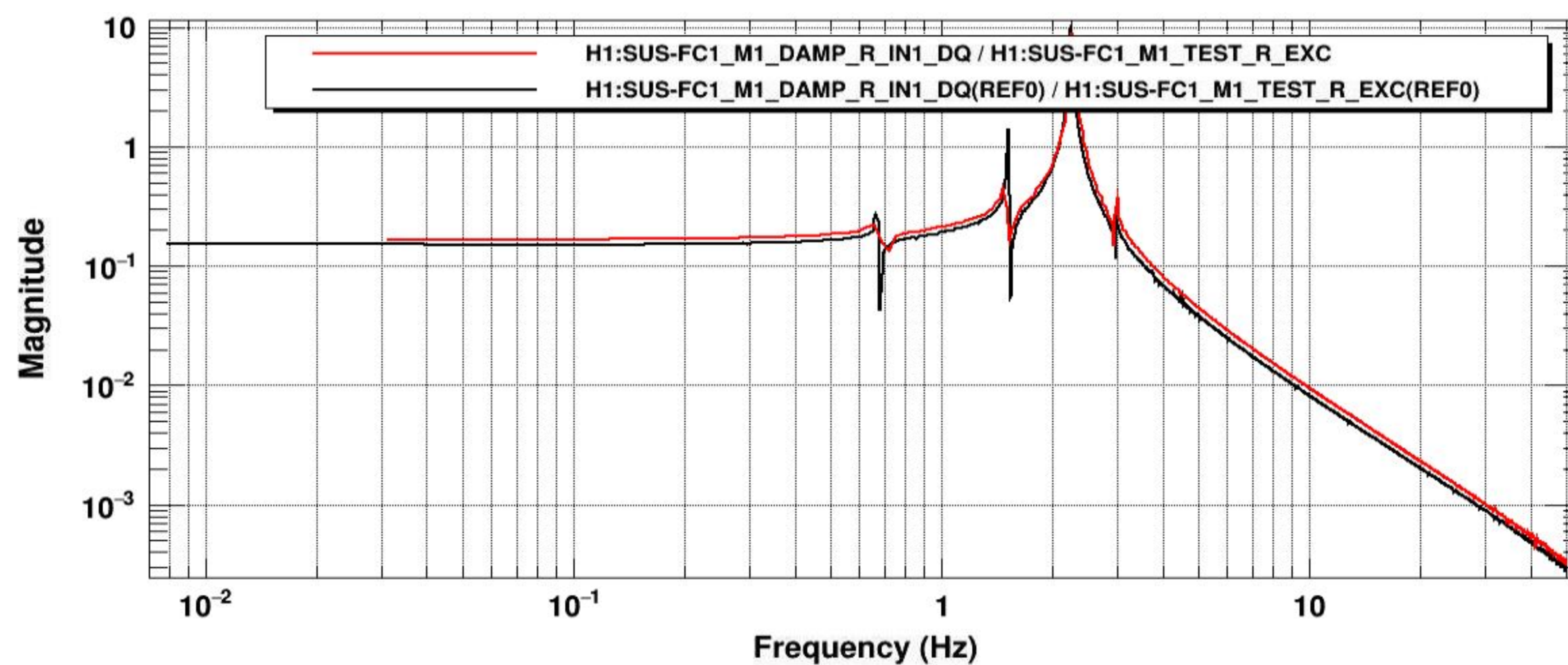
Transfer function
