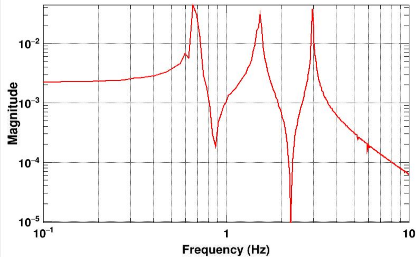
Transfer function
