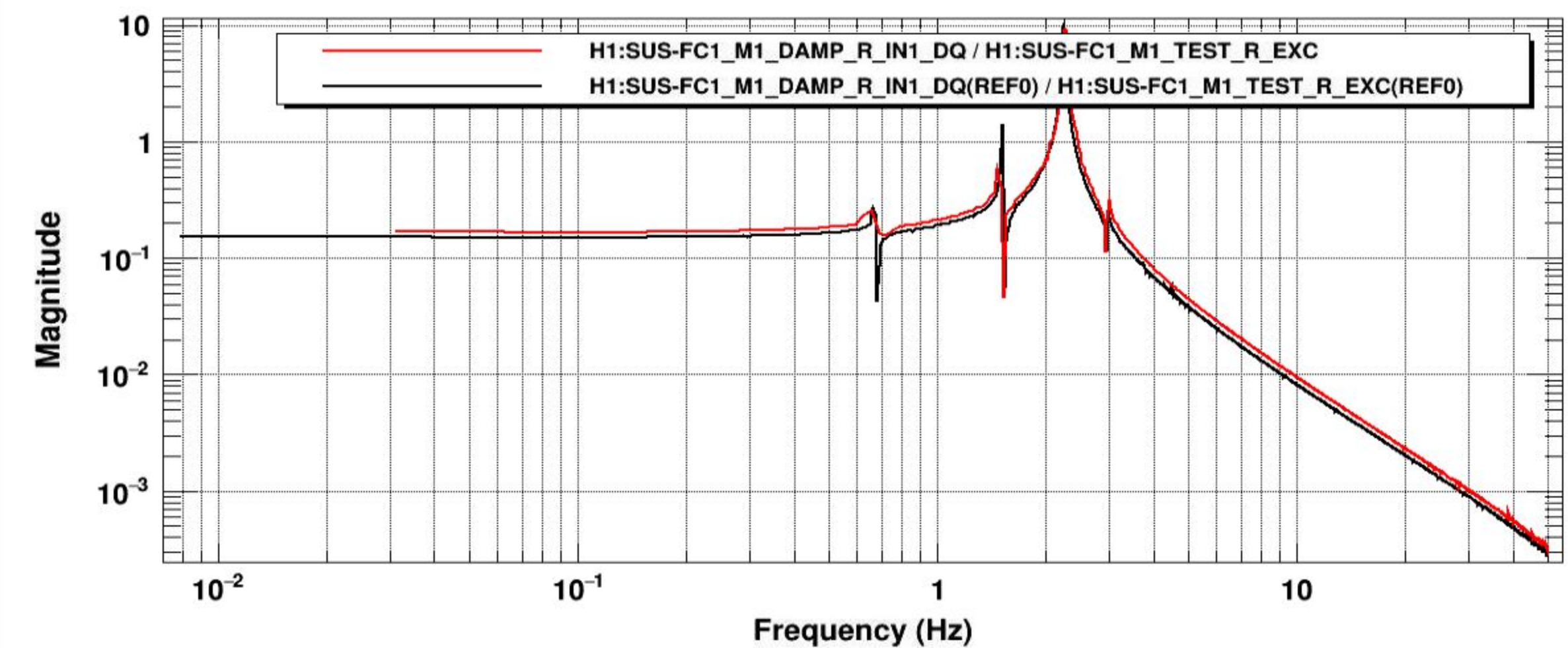
Transfer function
