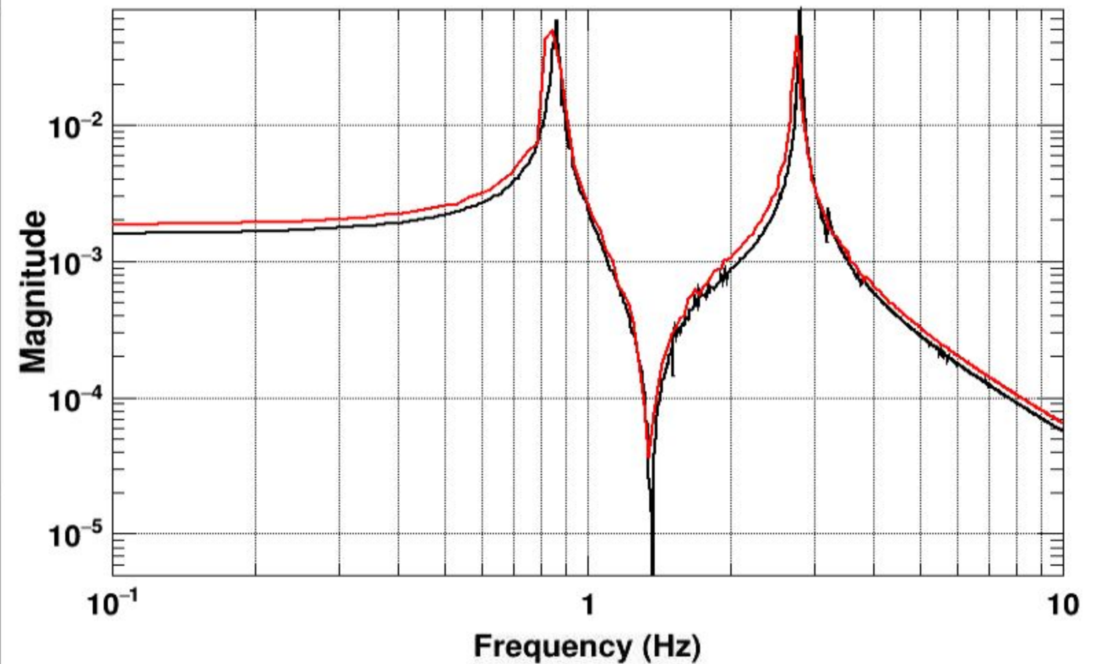
Transfer function
