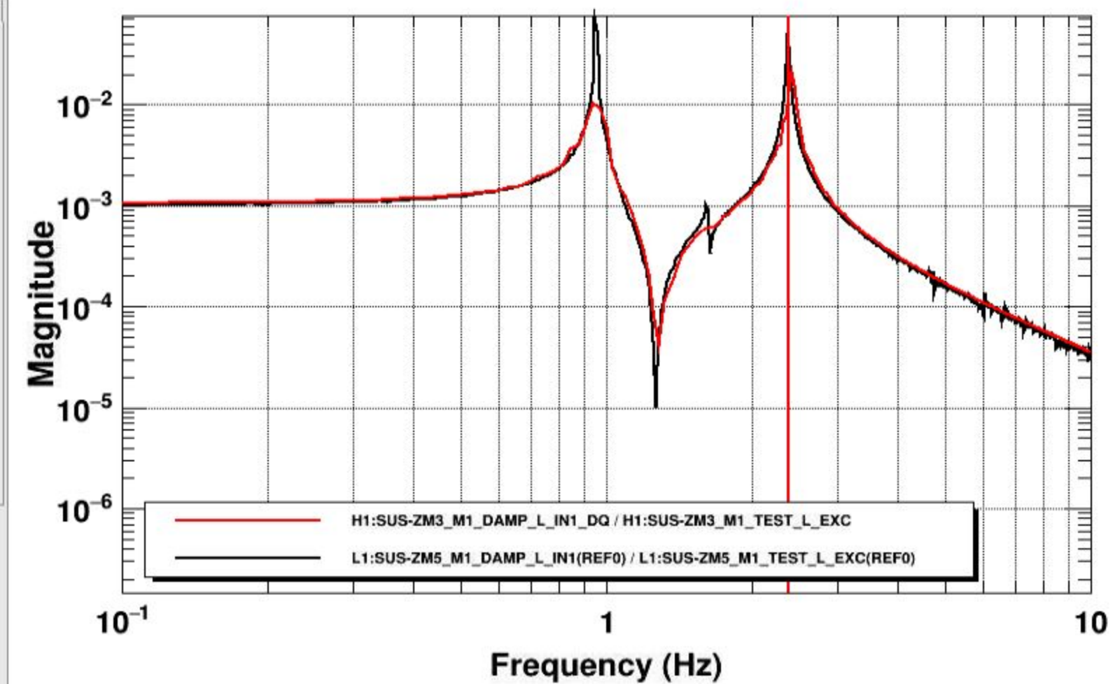
Transfer function
