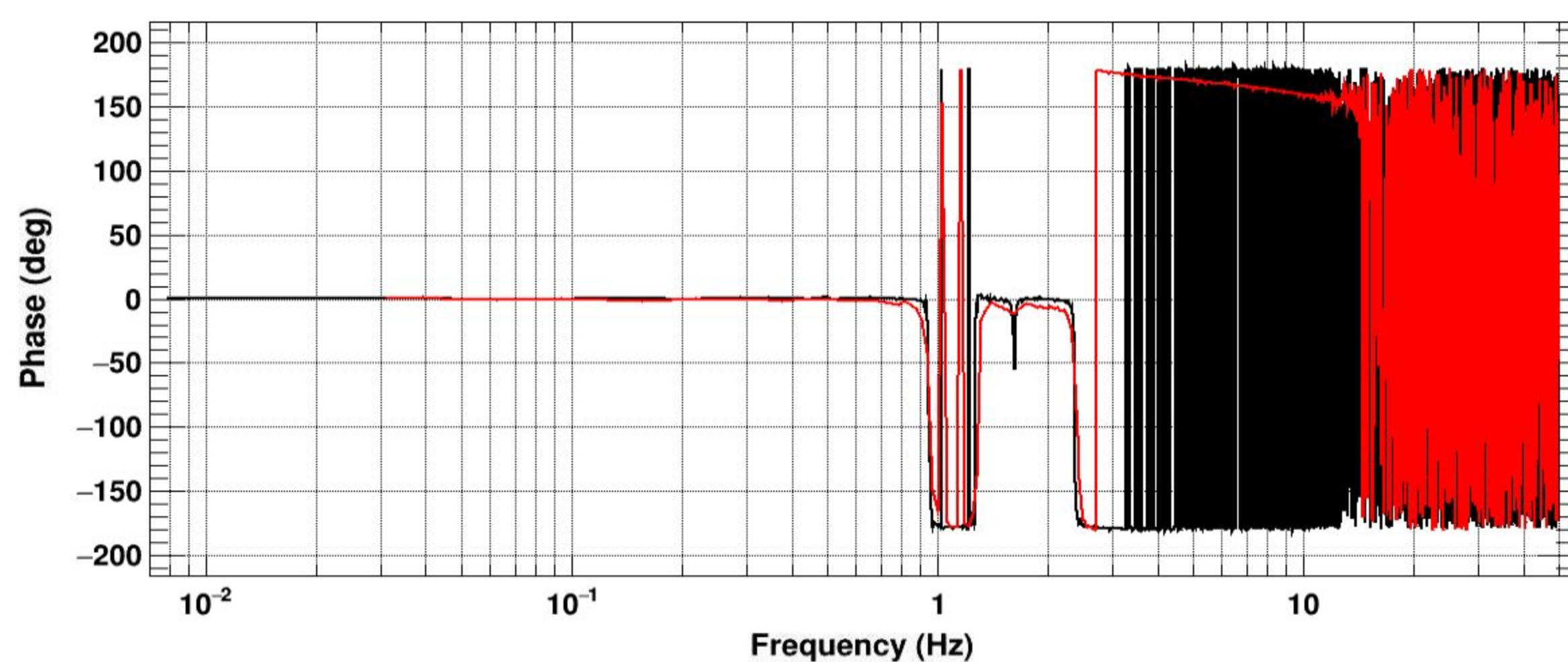
Transfer function
