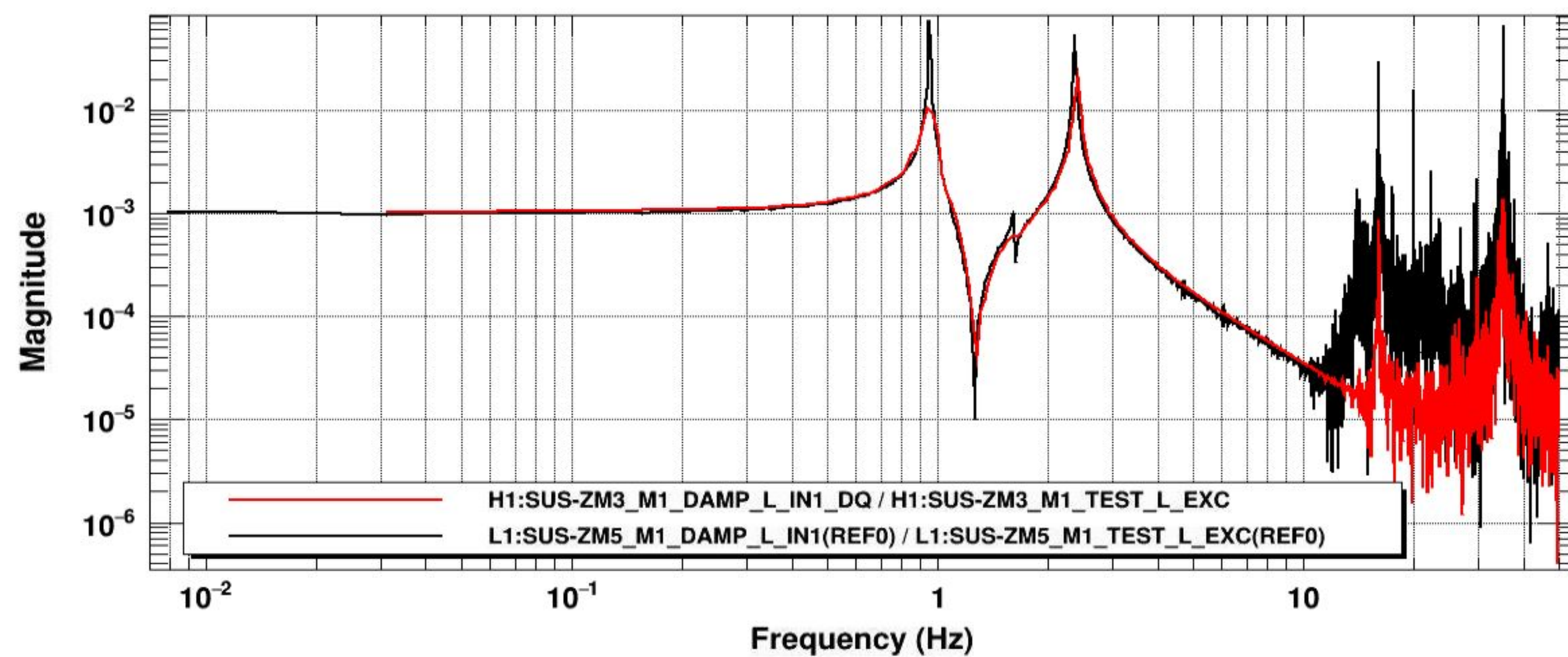
Transfer function
