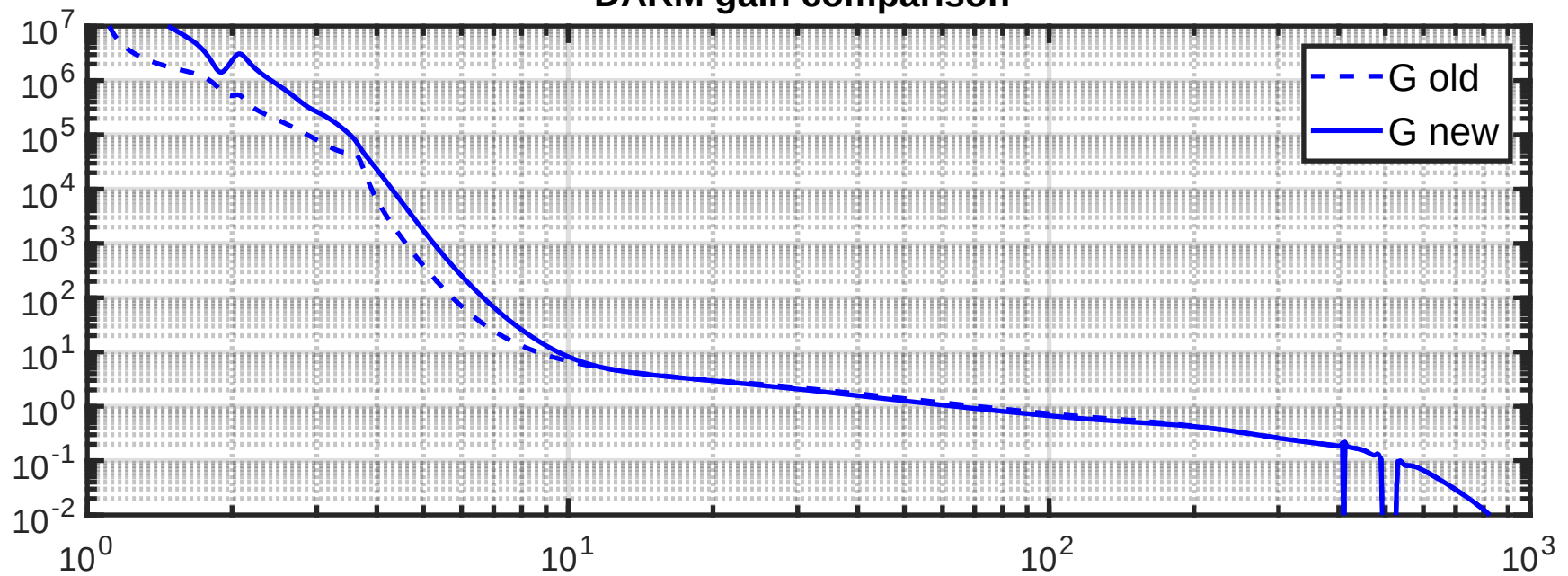
DARM gain comparison
