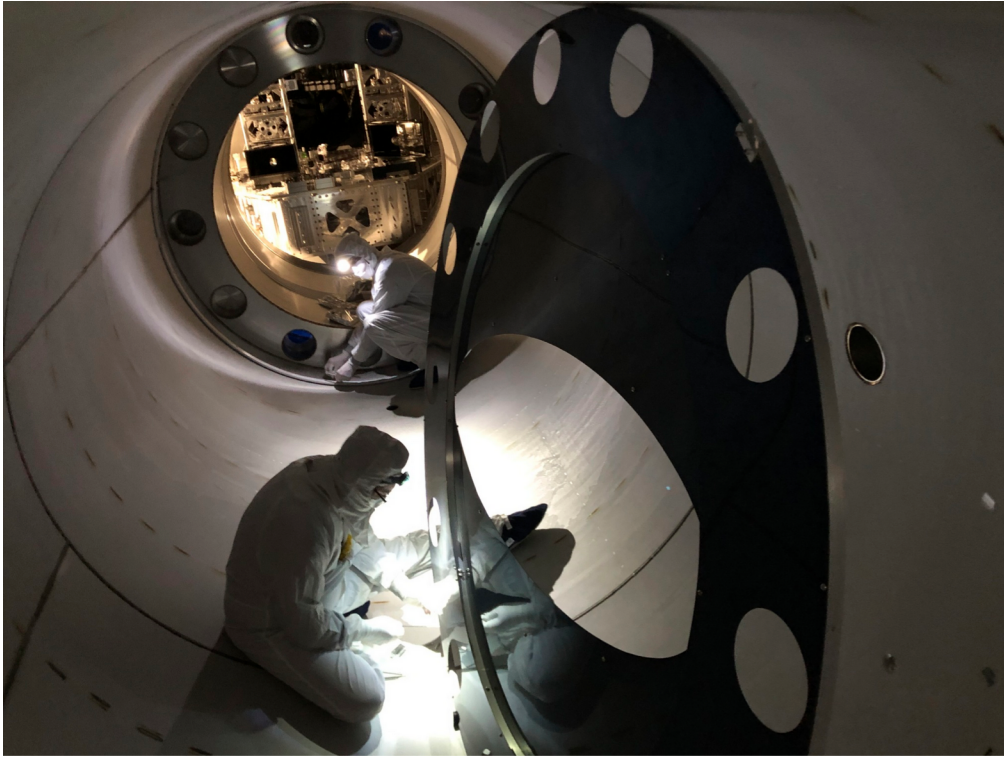
Mitchell and Robert working on baffle modification by HAM3 (photo: Corey)
