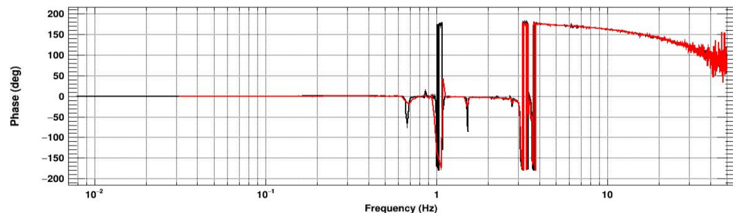
Transfer function
