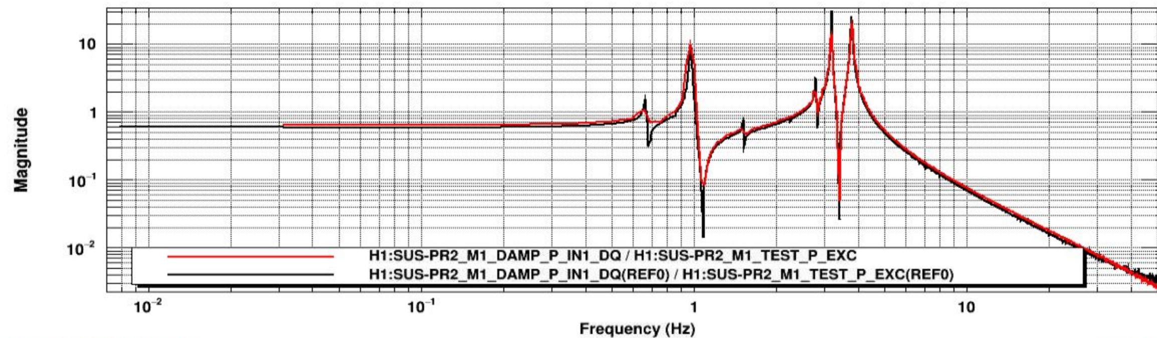
Transfer function
