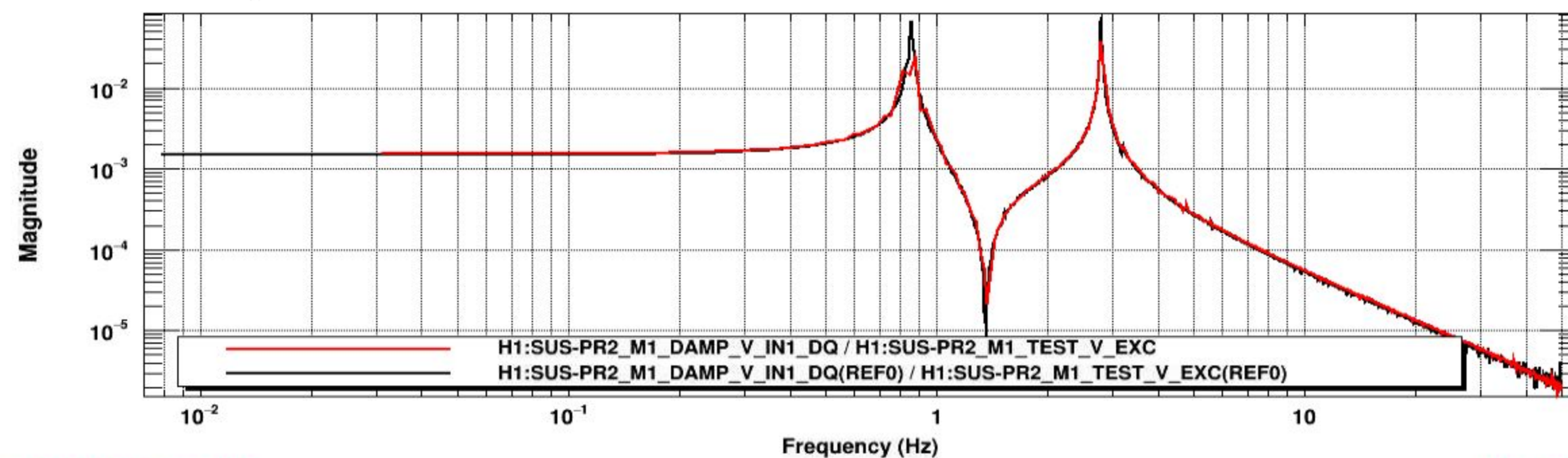
Transfer function
