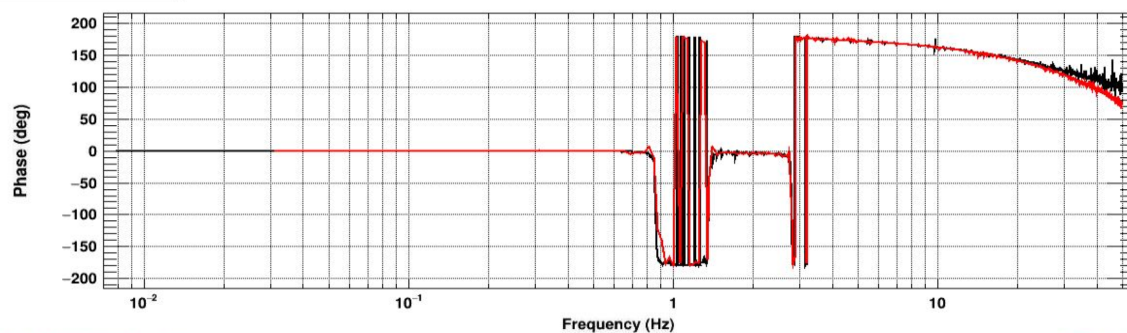
Transfer function
