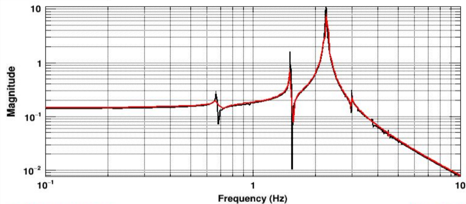
Transfer function
