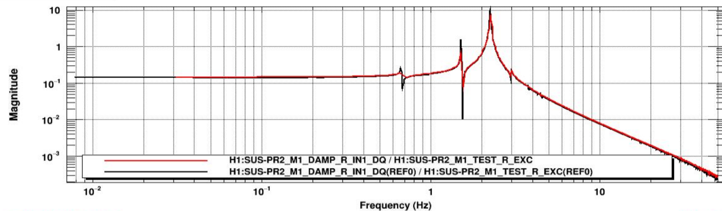
Transfer function
