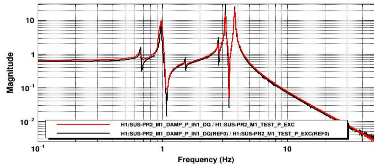
Transfer function
