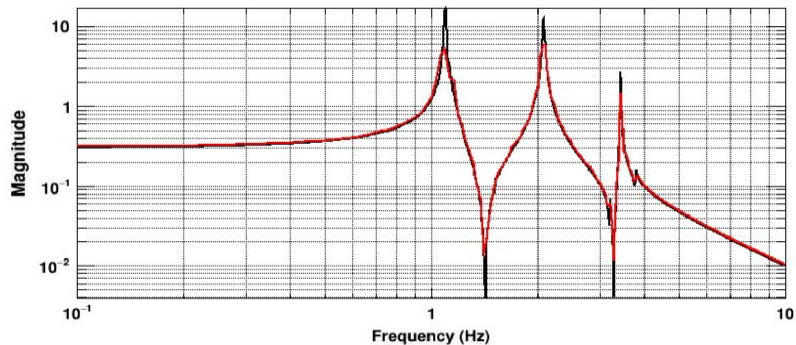
Transfer function
