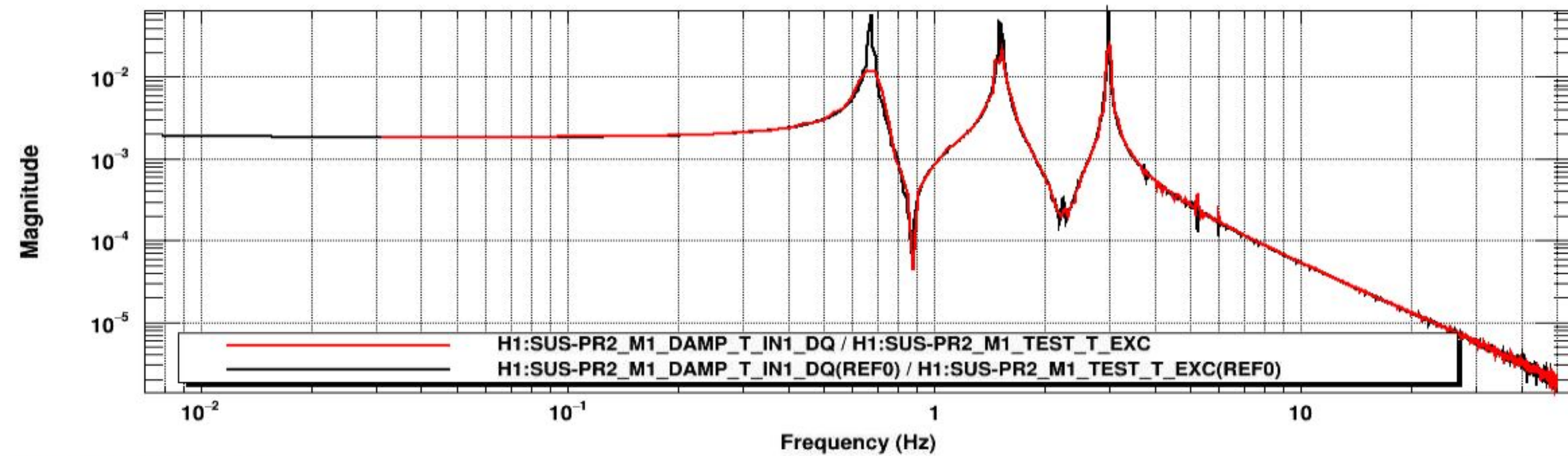
Transfer function
