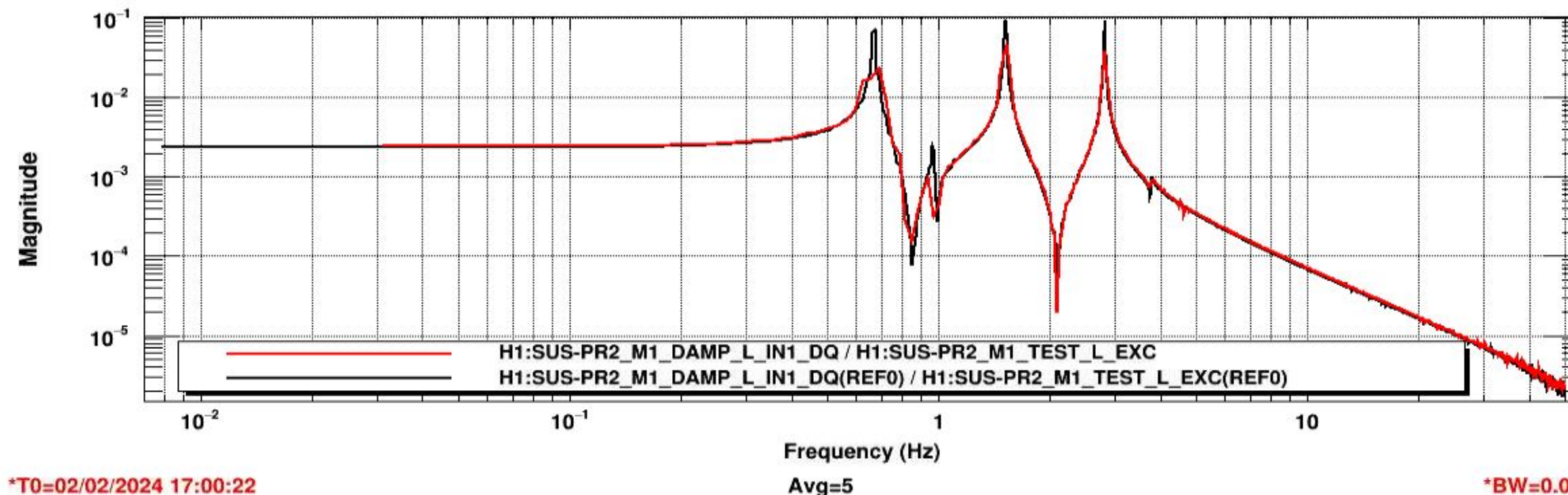
Transfer function
