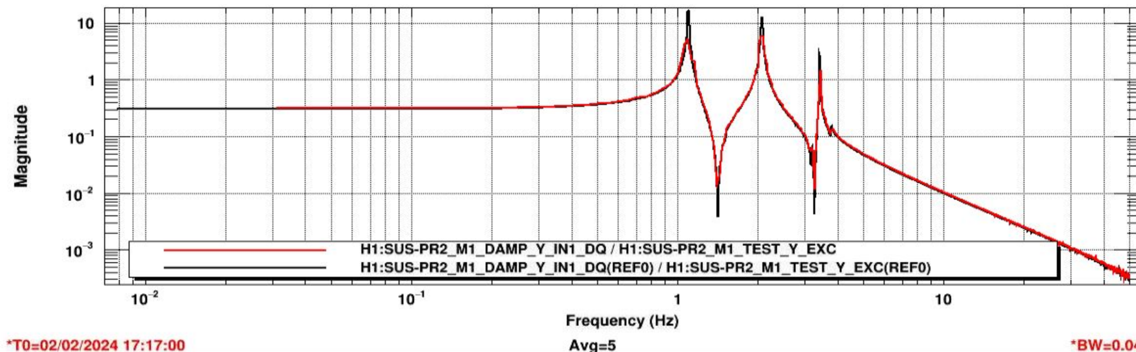
Transfer function
