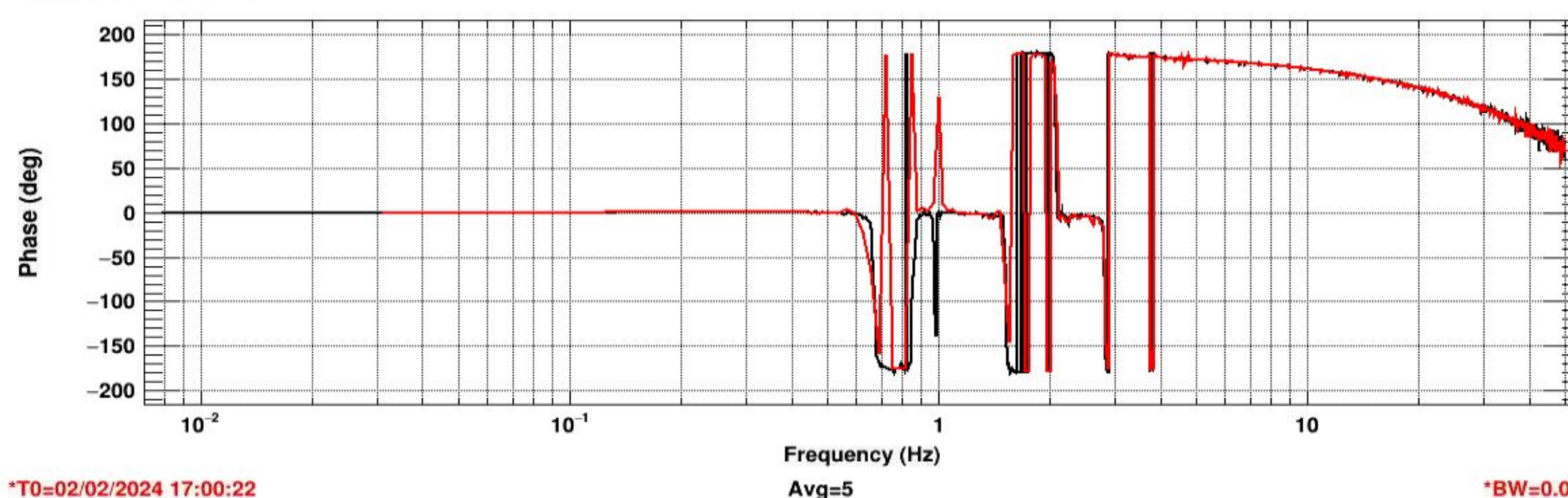
Transfer function
