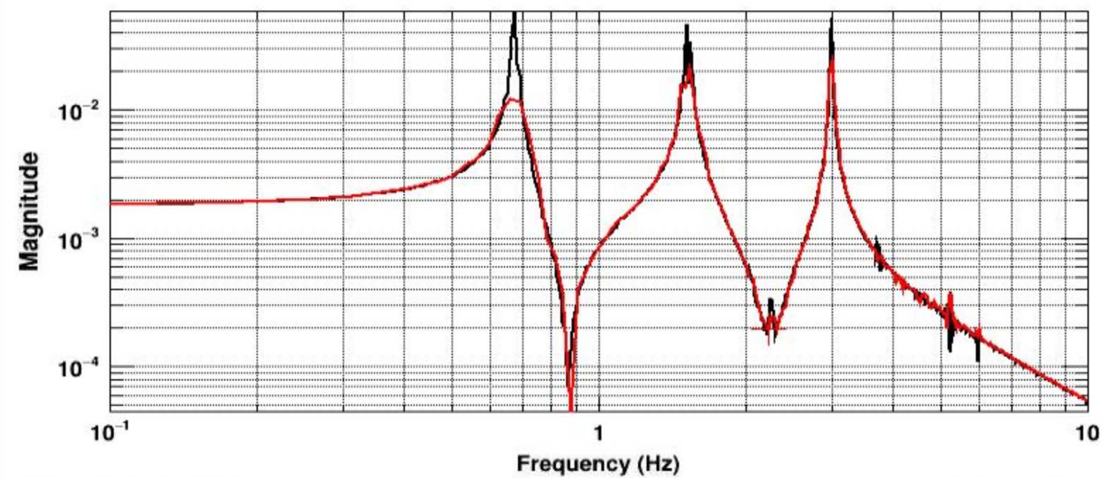
Transfer function
