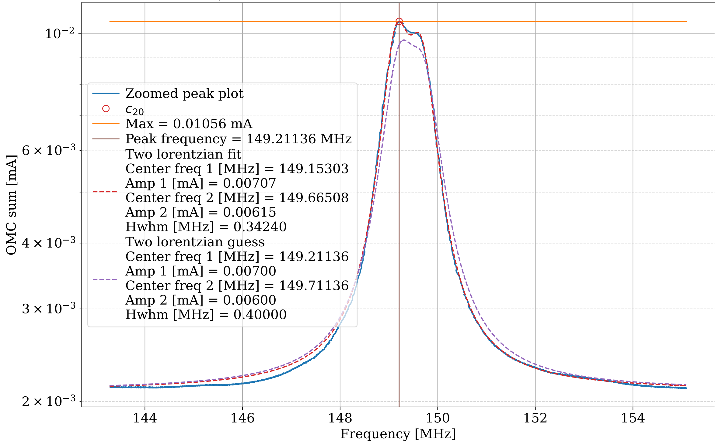
PSAMS 120/120, SQZ-OMC 1st scan zoomed at carrier + 20, HWHM = 0.40000 MHz
