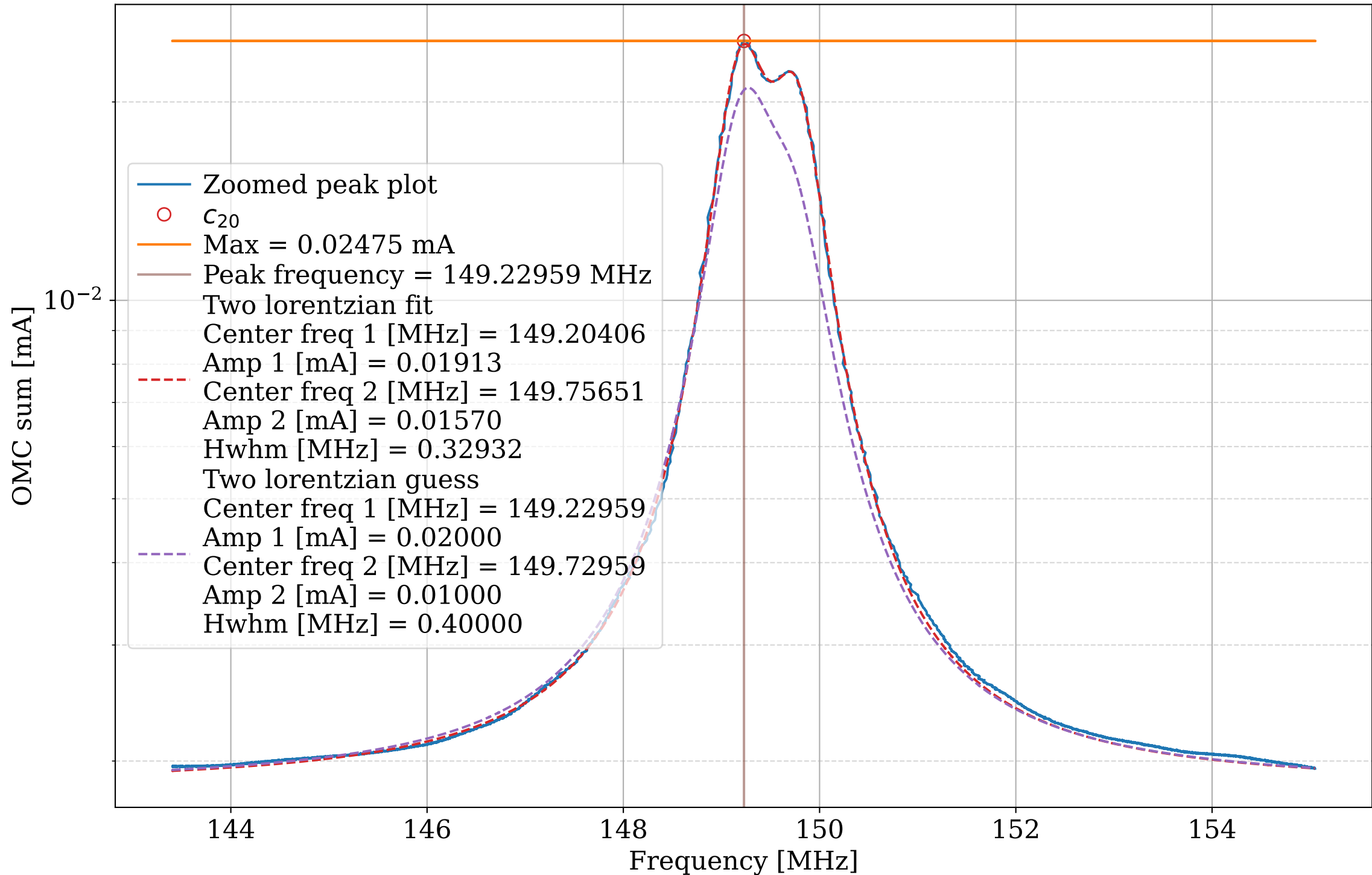
PSAMS 200/200, SQZ-OMC 2nd scan zoomed at carrier + 20, HWHM = 0.40000 MHz
