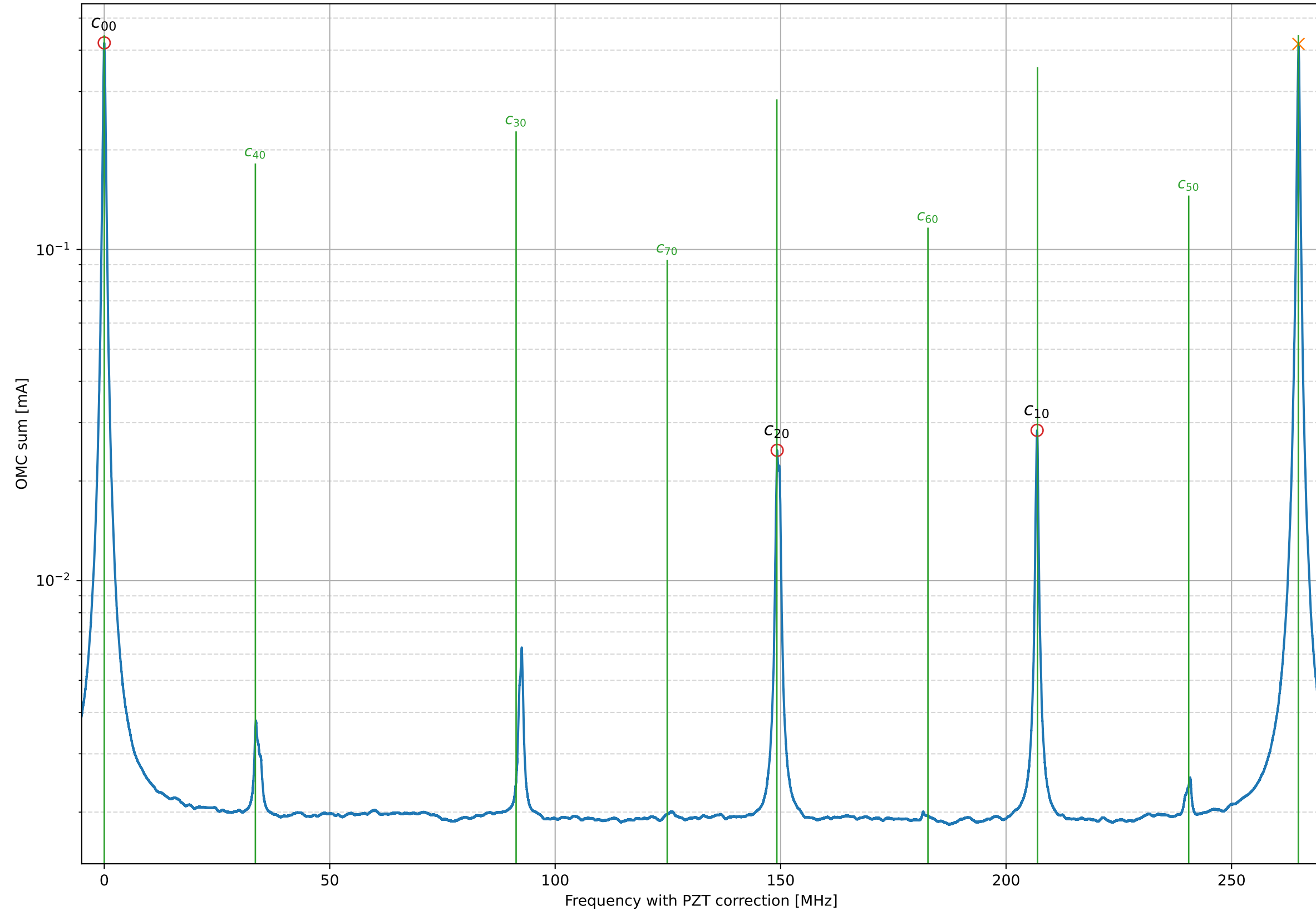
PSAMS 200/200, SQZ-OMC 2nd scan
