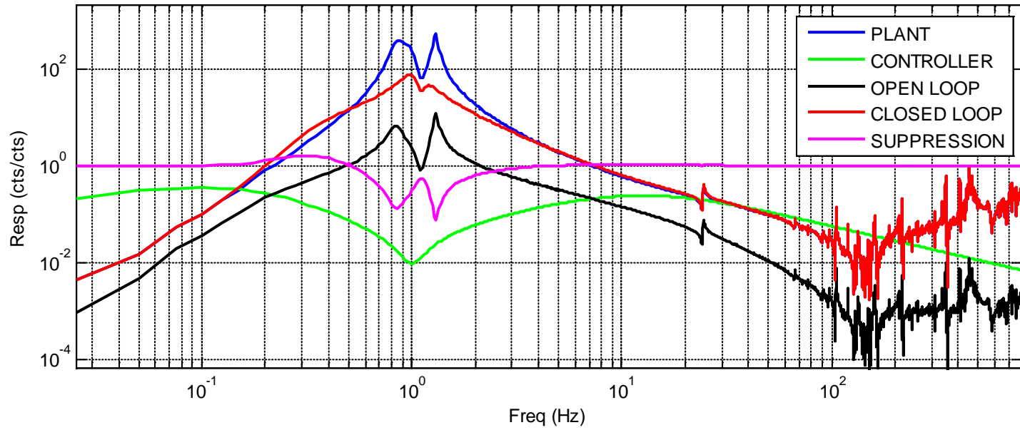
H1 Damping Loop
