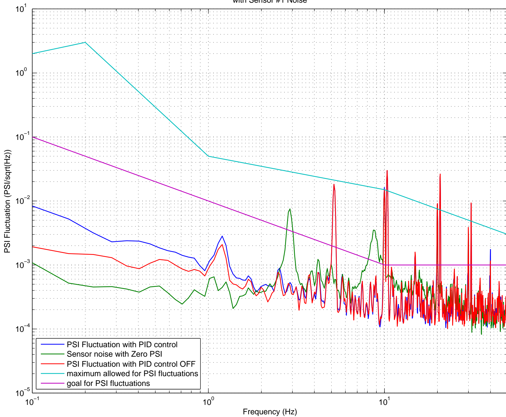
PID Control ON, OFF, and Zero PSI Compare HEPI Pump Servo ASD of PSI fluctuations with Sensor #1 Noise
