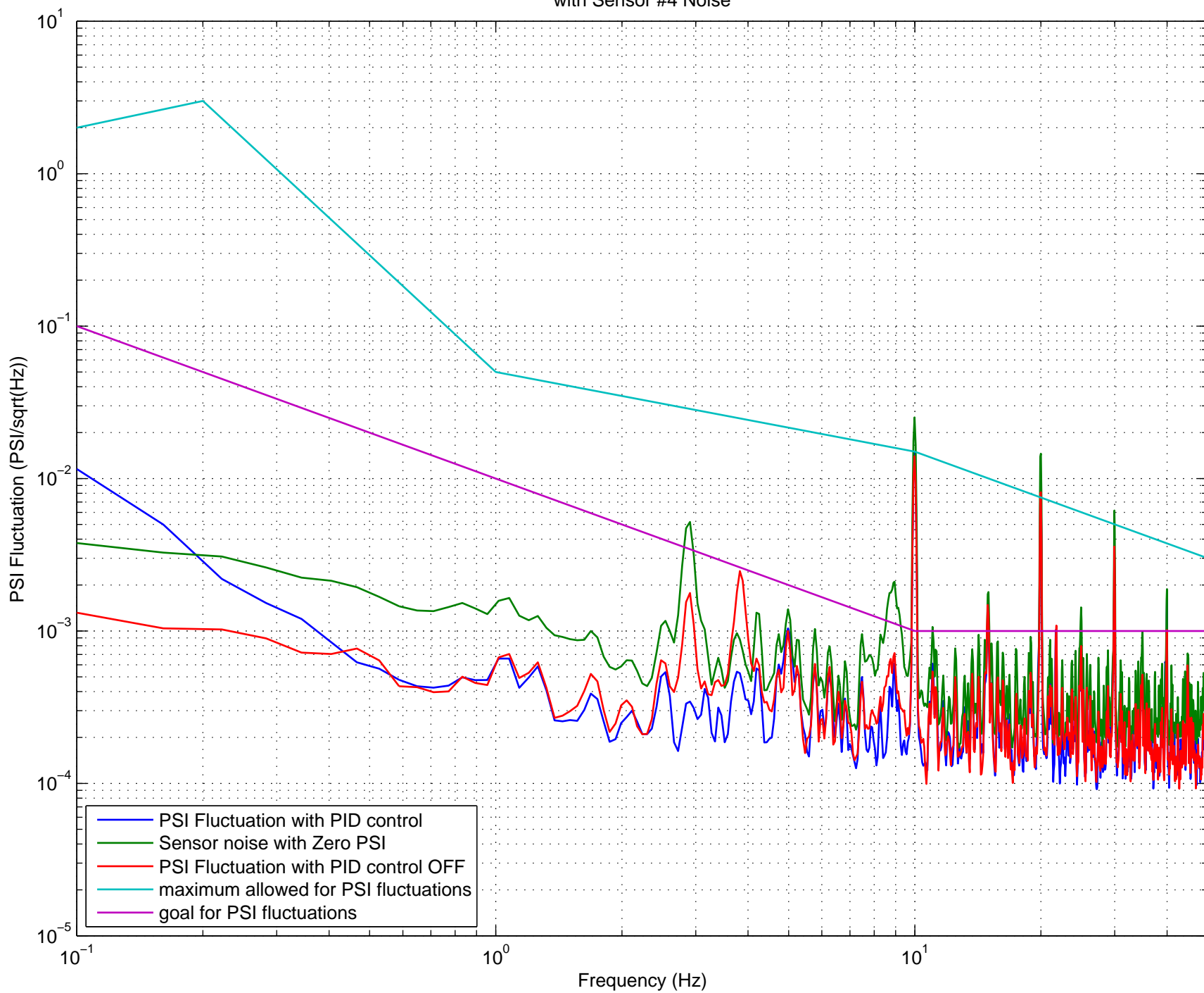
PID Control ON, OFF, and Zero PSI Compare HEPI Pump Servo ASD of PSI fluctuations with Sensor #4 Noise
