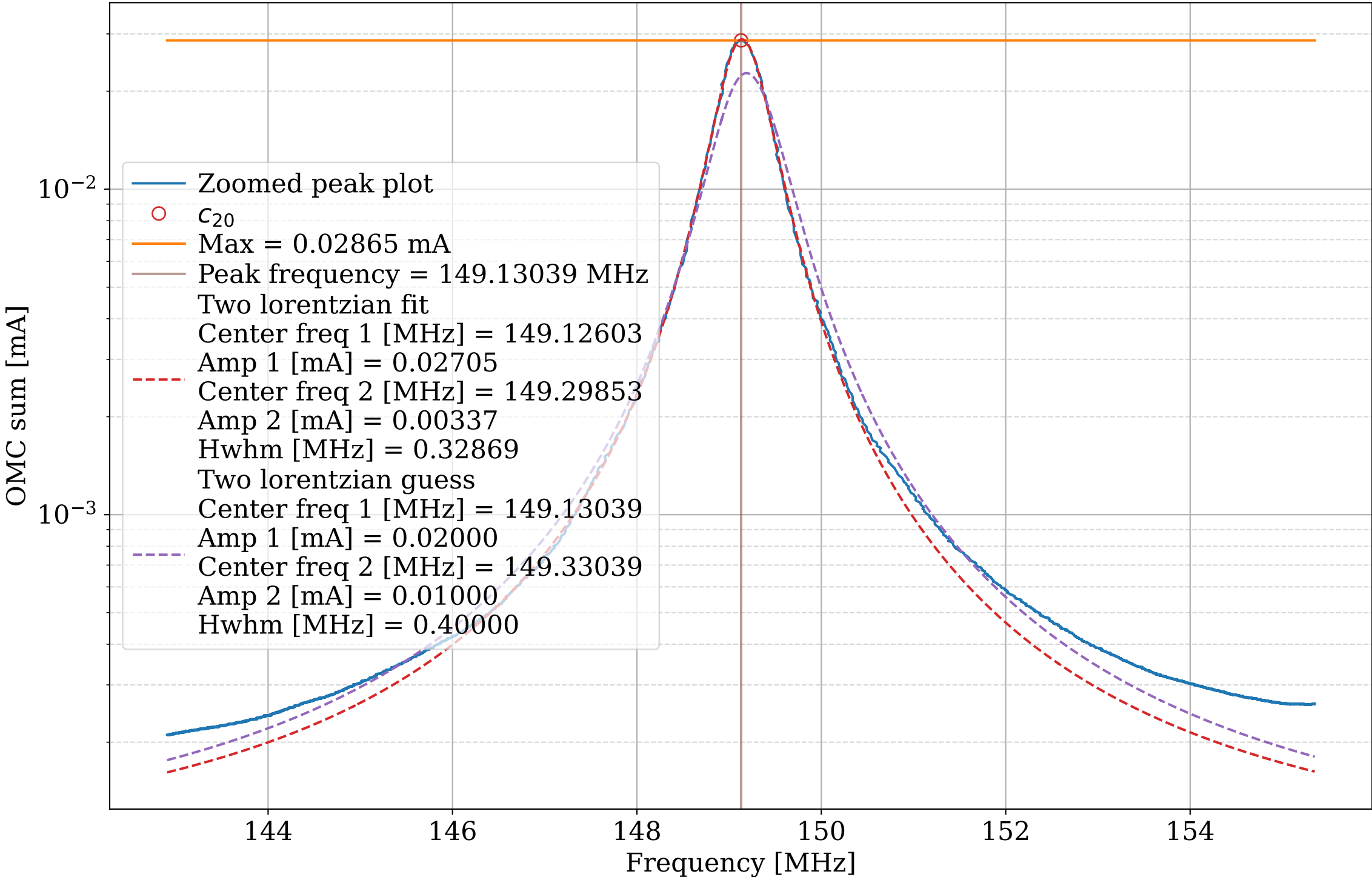
PSAMS 175/100, SQZ-OMC scan post O4 comm break zoomed at carrier + 20, HWHM = 0.40000 MHz
