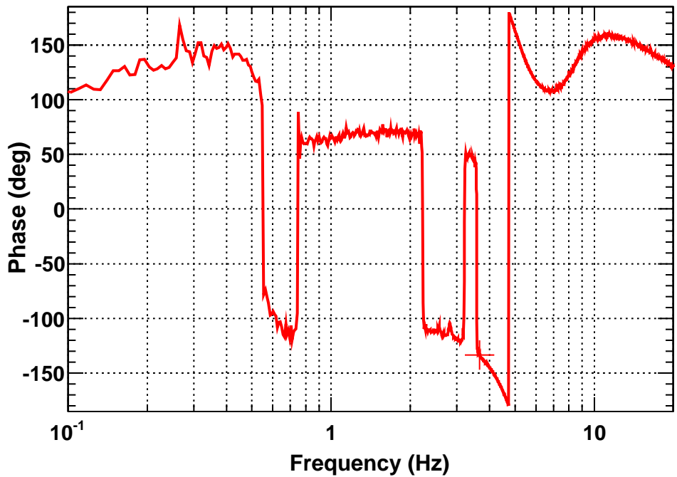
Transfer function
