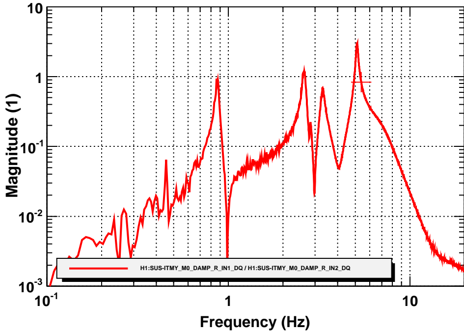
Transfer function
