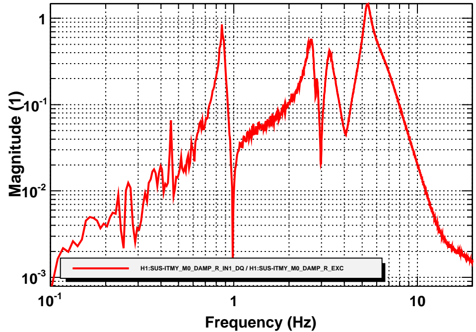
Transfer function
