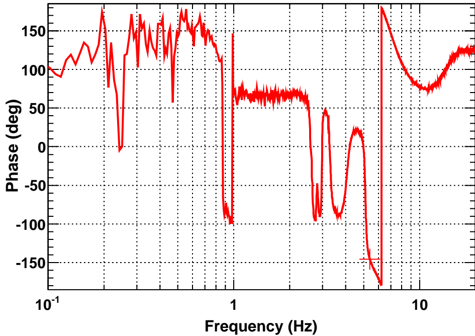
Transfer function
