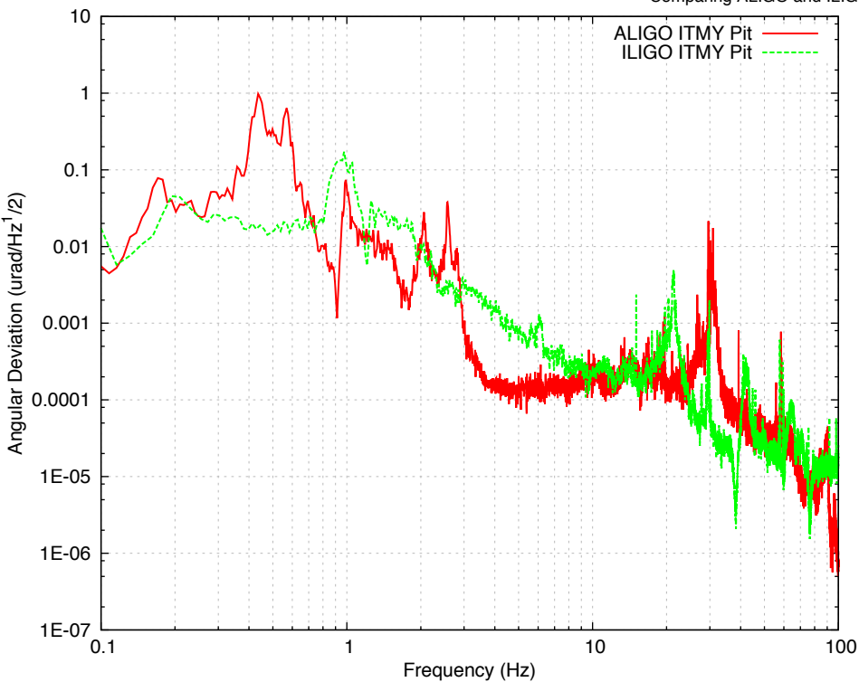
Comparing ALIGO and ILIGO ITMY Optical Lever Spectra
