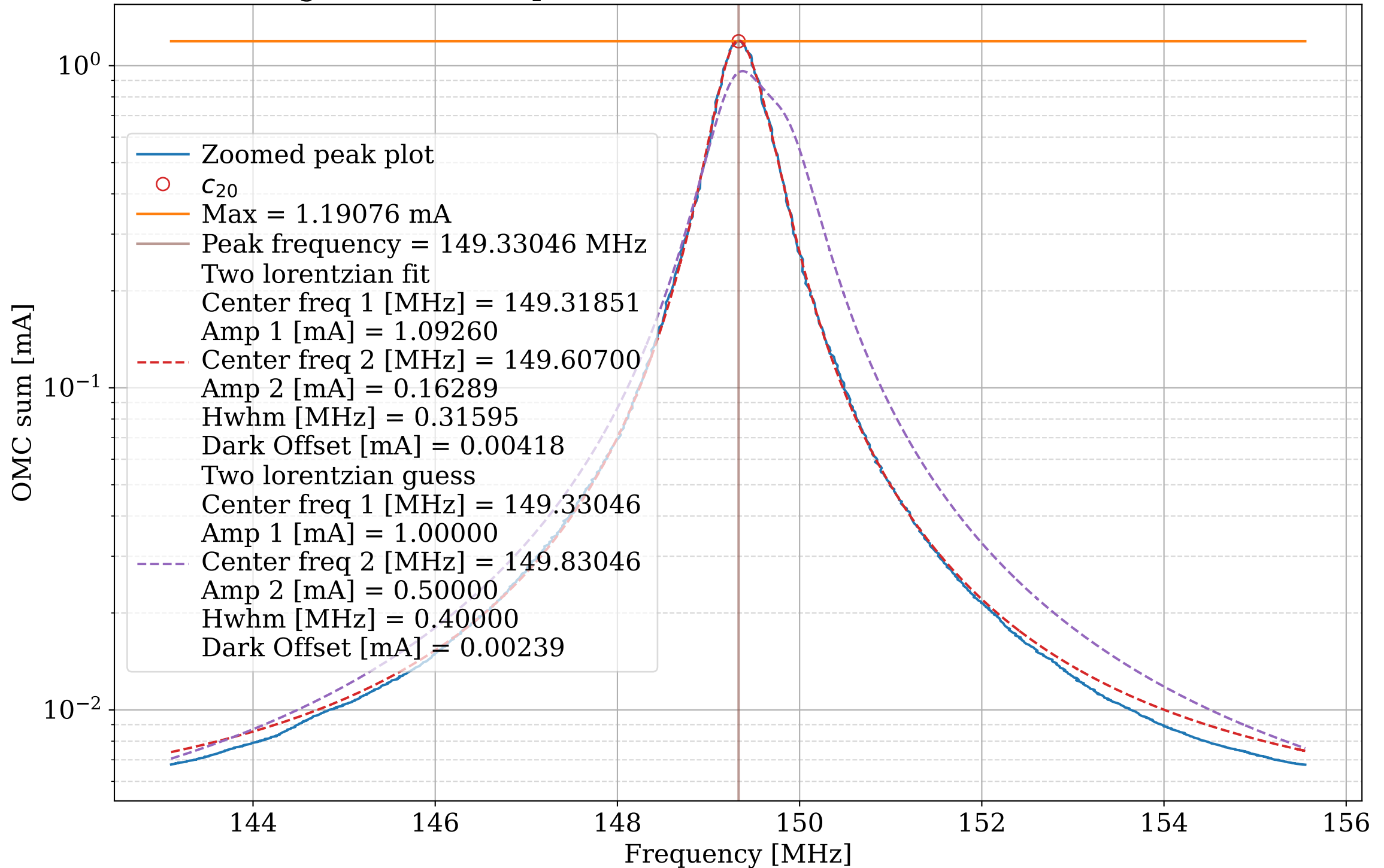
PSL scan, old alignment from April 22nd zoomed at carrier + 20, HWHM = 0.40000 MHz
