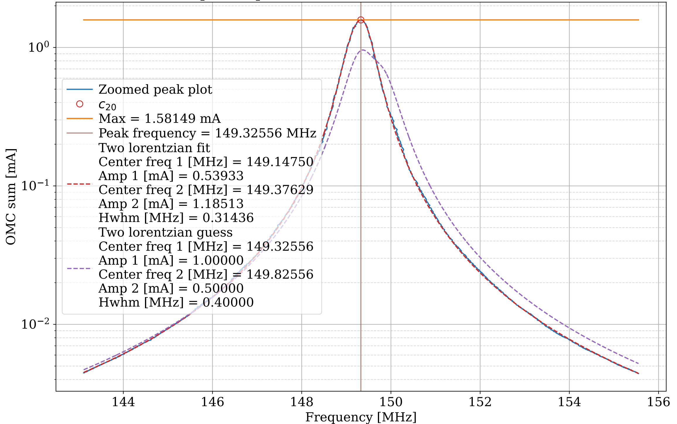
Cold OM2, 10W PSL, pre-output loss zoomed at carrier + 20, HWHM = 0.40000 MHz
