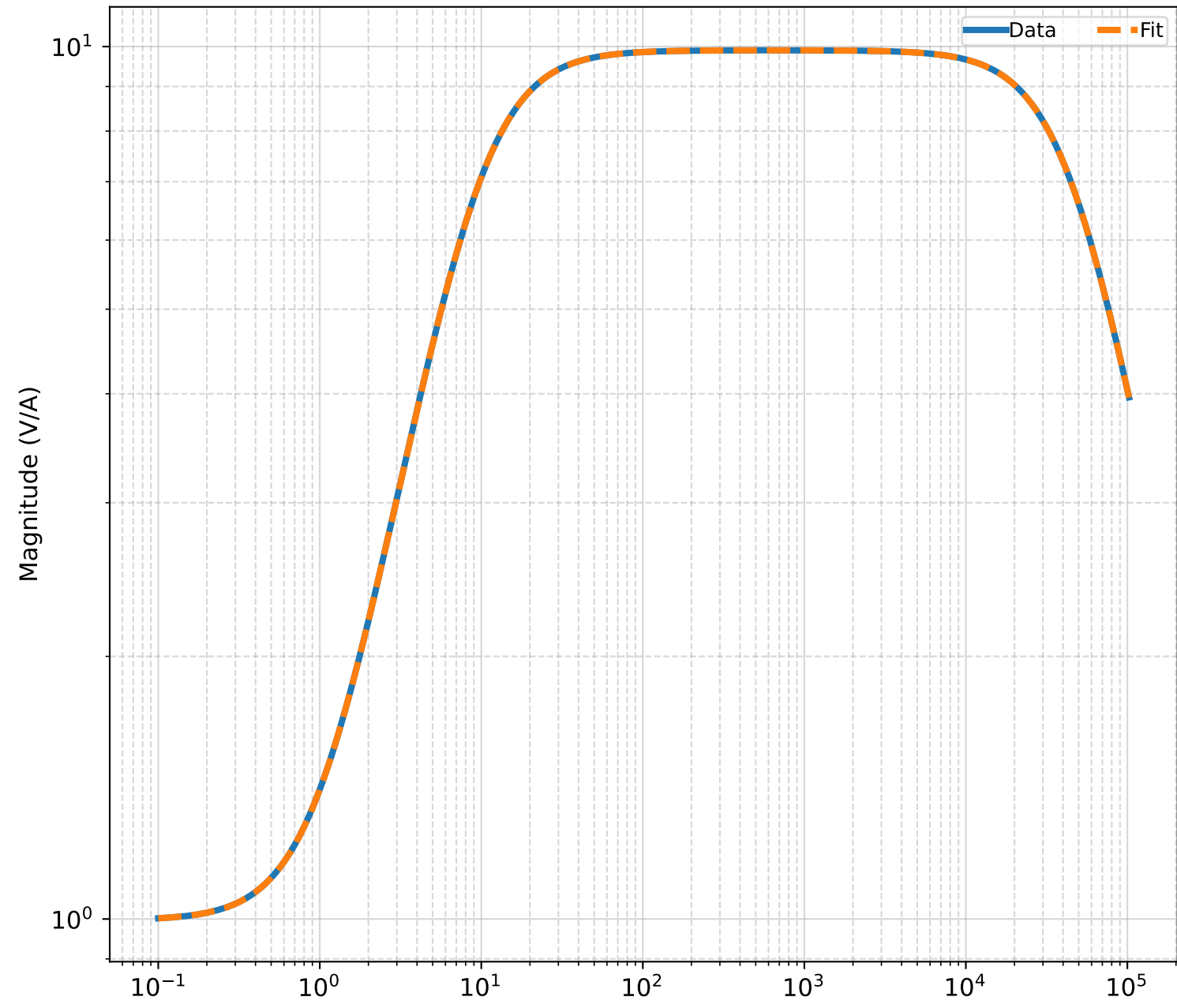
2024-05-23_OMCDCPDWhiteningOMCA_OMCA_DCPDA_WhiteningON_0p1to102p4e3Hz_1Vsrcinput
