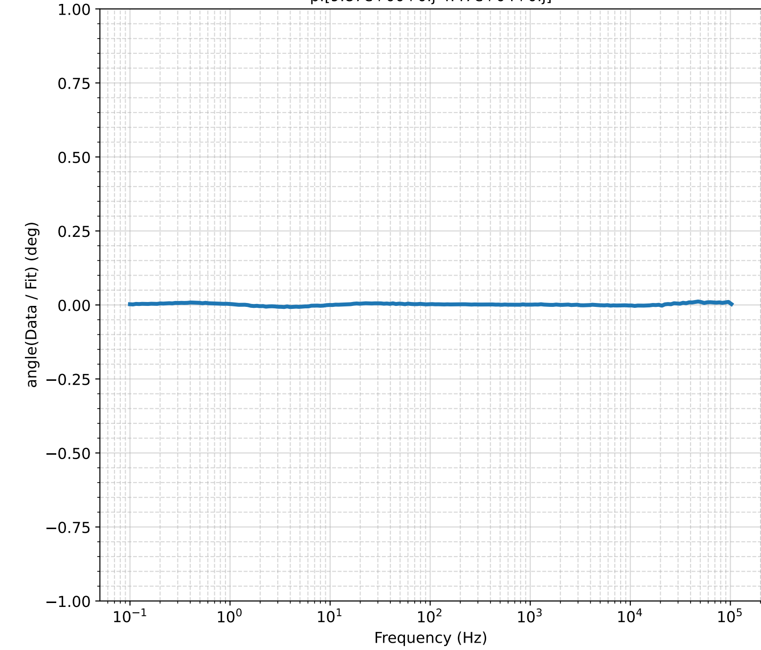
Residual angle (Measured Data / Fit) p:[9.87e+00+0.j \ 4.47e+04+0.j]
