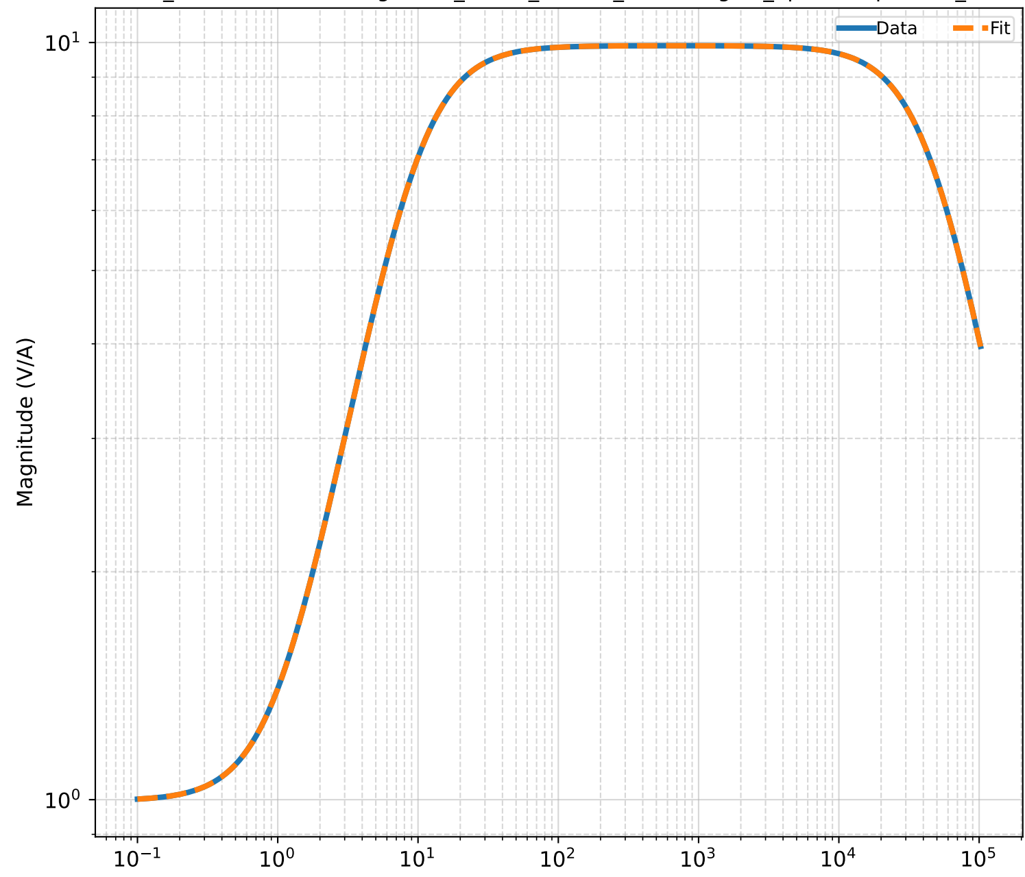
2024-05-23_OMCDCPDWhiteningOMCA_OMCA_DCPDB_WhiteningON_0p1to102p4e3Hz_1Vsrcinput
