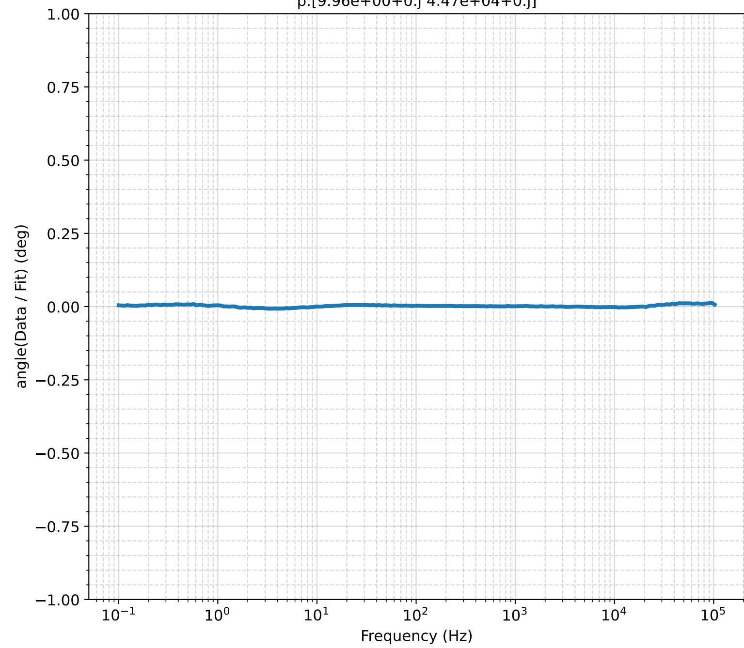
Residual angle (Measured Data / Fit) p:[9.96e+00+0.j \ 4.47e+04+0.j]
