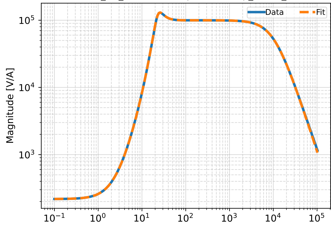
20240611_H1_DCPDTransimpedanceAmp_OMCA_DCPDA
