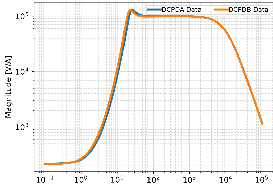
H1 OMCA DCPD Transimpedance
