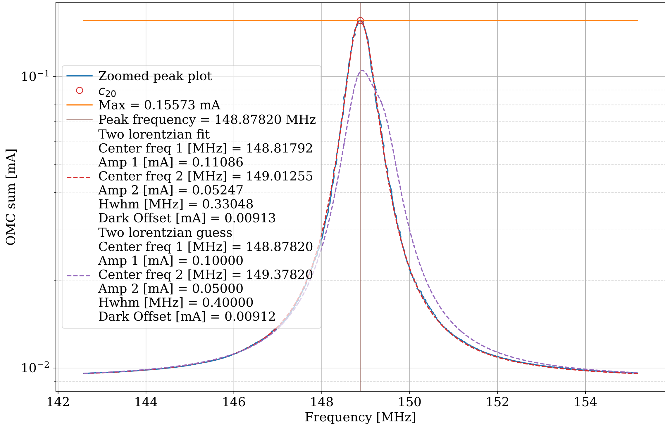
OM2 hot and thermalised, 2W PSL zoomed at carrier + 20, HWHM = 0.40000 MHz
