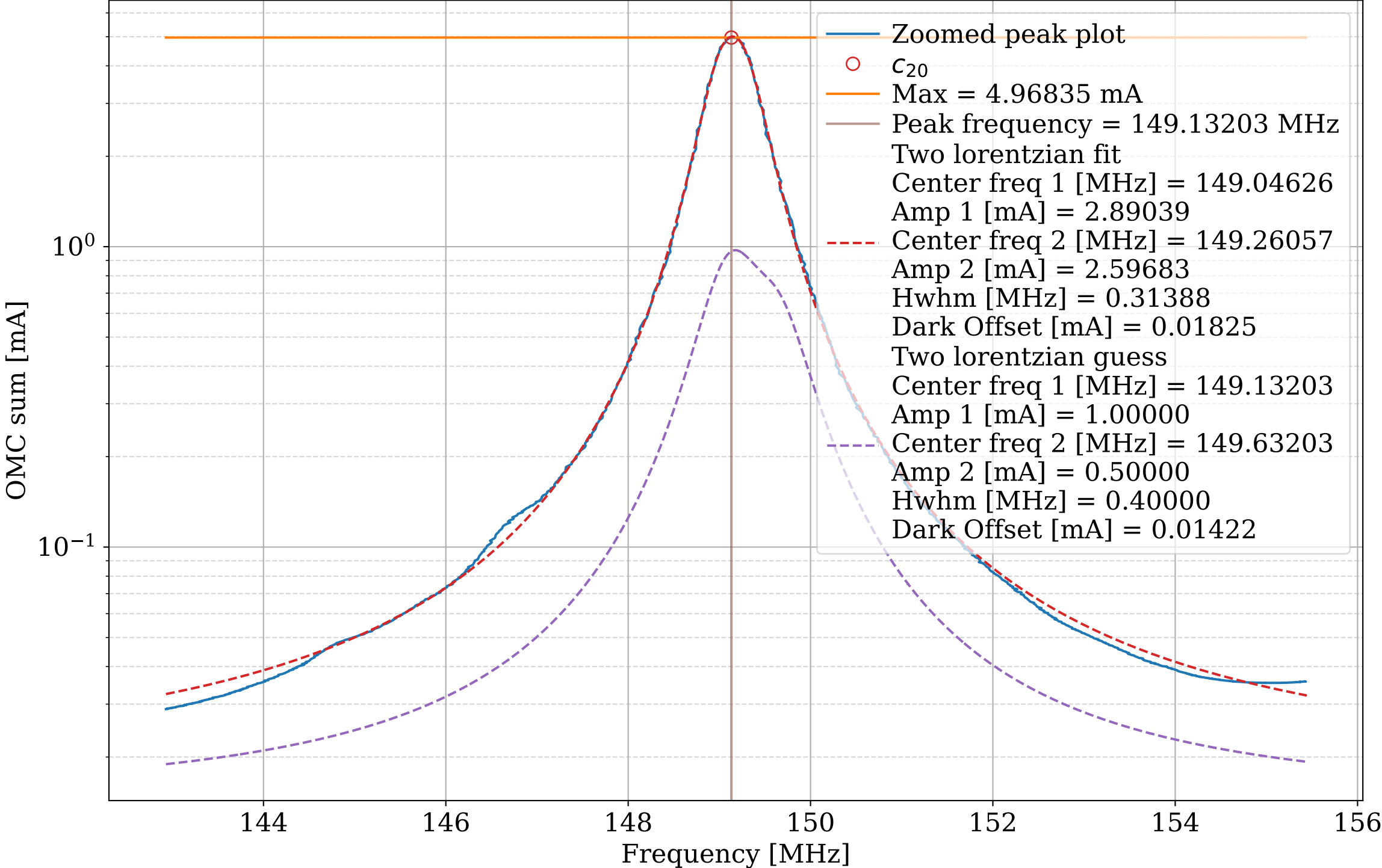
OMC Scan before OFI move on 6th June, 10 W lock. zoomed at carrier + 20, HWHM = 0.40000 MHz
