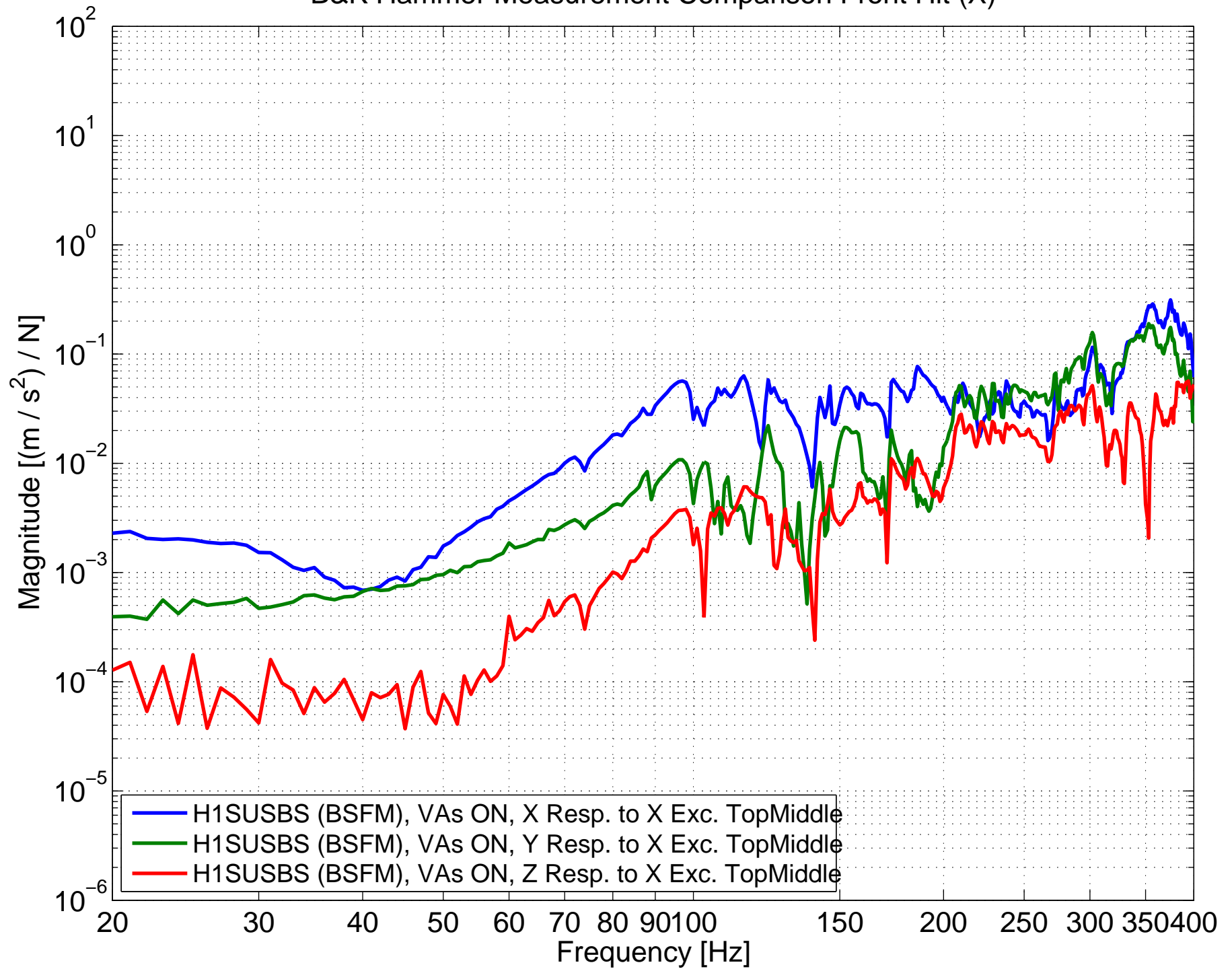
B&K Hammer Measurement Comparison Front Hit (X)
