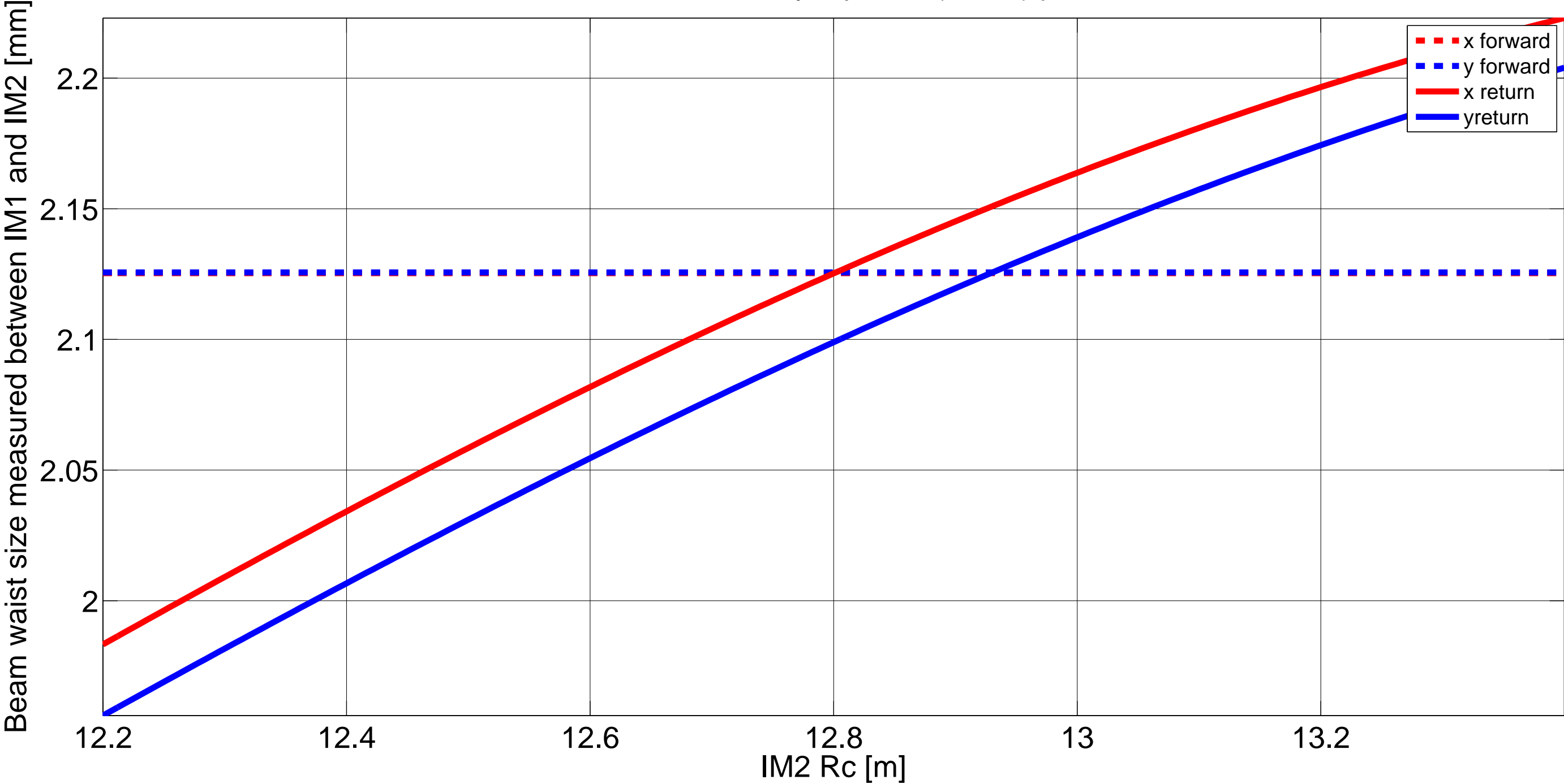
Beam waist radius at Faraday rejected (REFL) port with IM2 Rc
