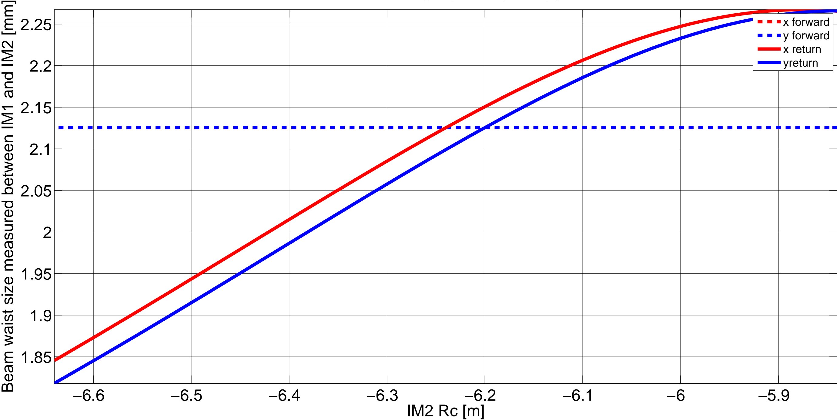
Beam waist radius at Faraday rejected (REFL) port with IM3 Rc
