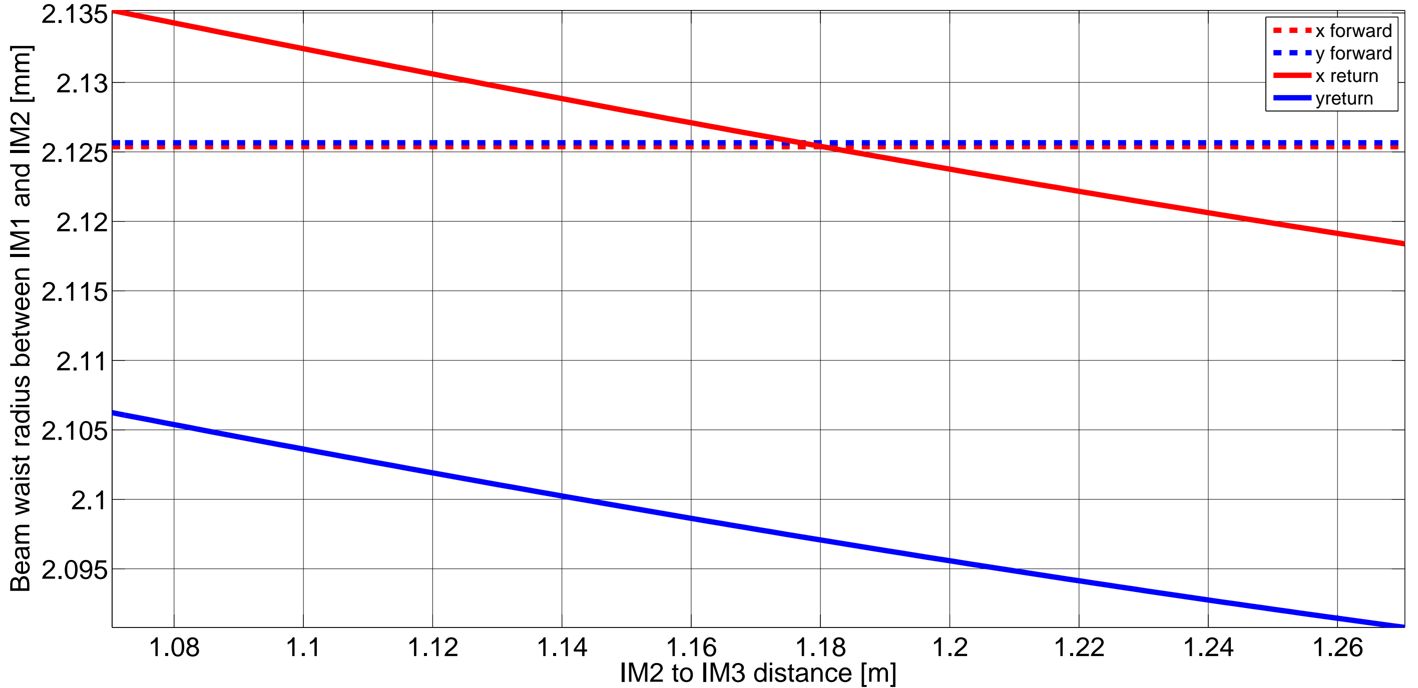
Beam waist radius at Faraday rejected (REFL) port with IM2 to IM3 distance
