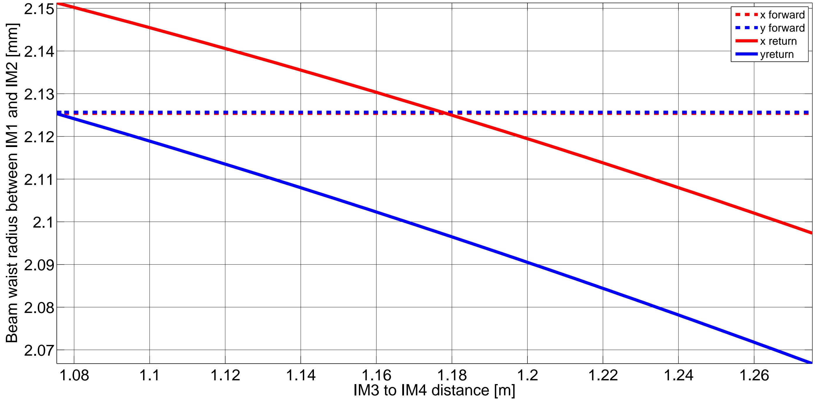
Beam waist radius at Faraday rejected (REFL) port with IM3 to IM4 distance
