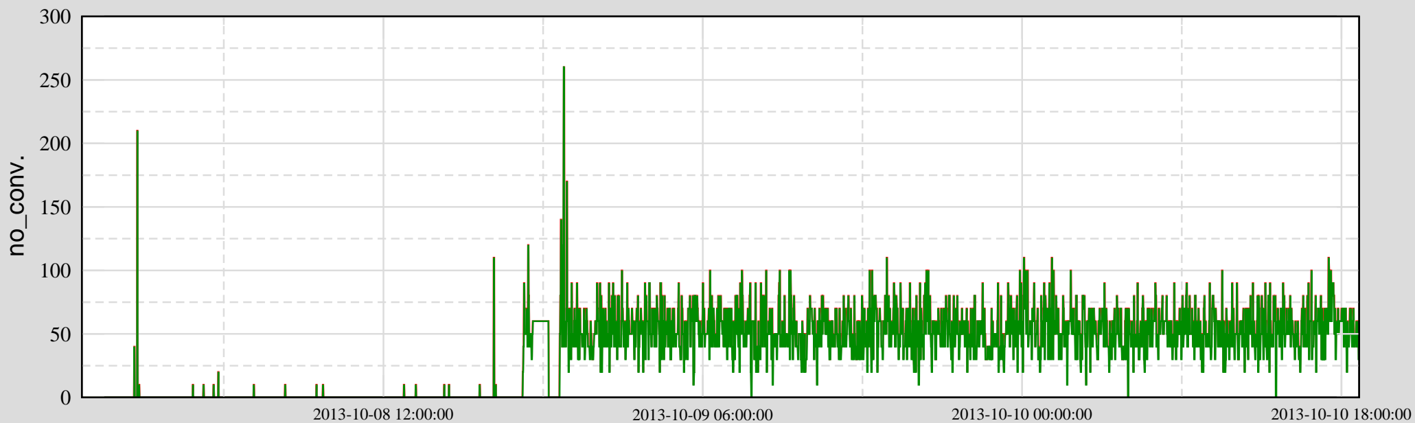
Ch 5: H0:PEM-EX_DUST_VEA1_300NM_PCF
