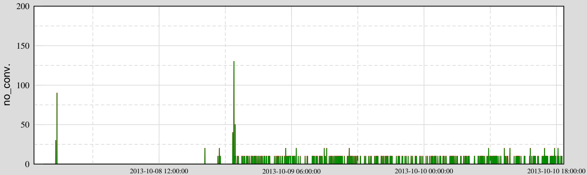
Ch 6: H0:PEM-EX_DUST_VEA1_500NM_PCF
