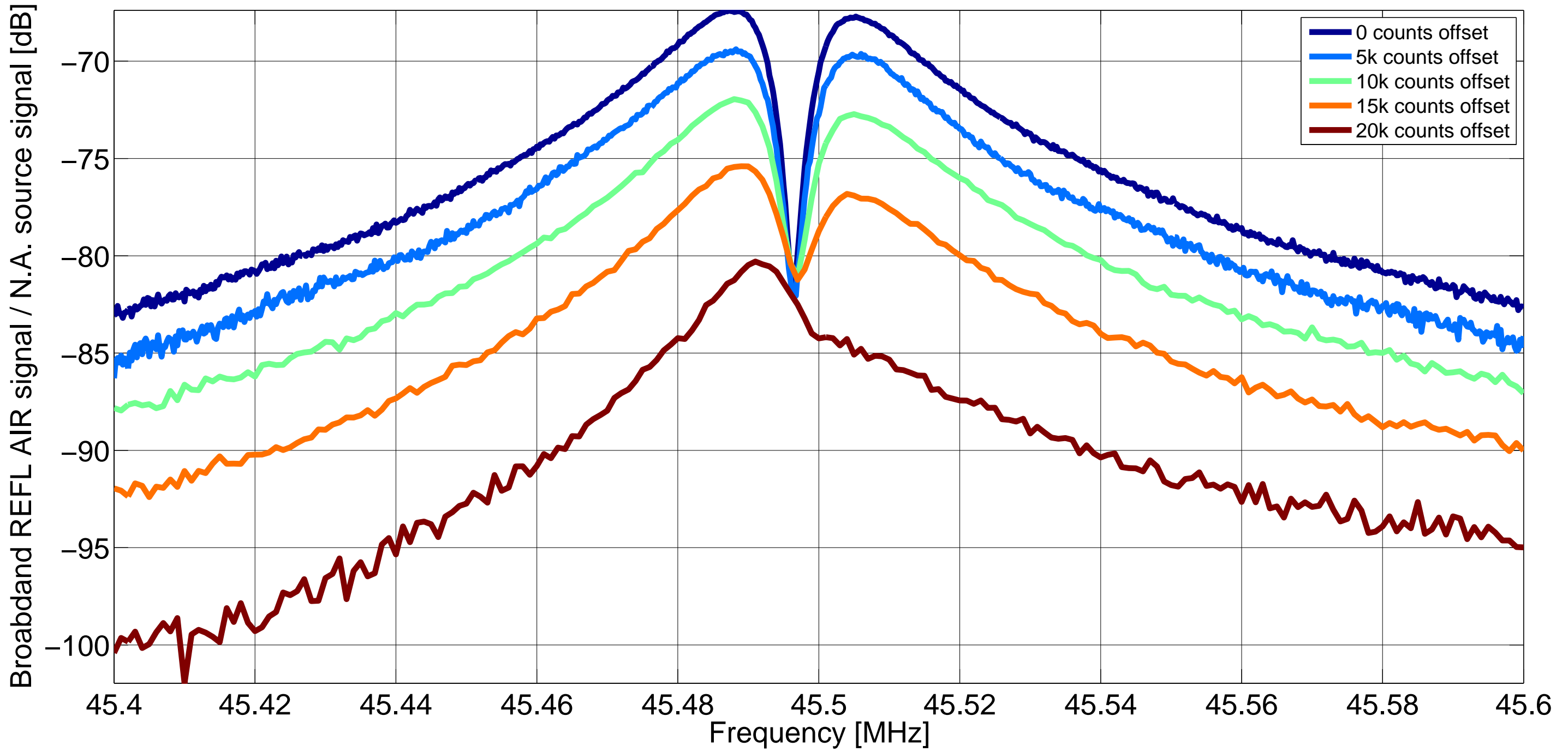
45.5 MHz sideband sweep for different PDH offsets
