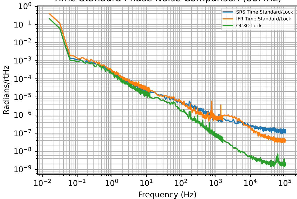
Time Standard Phase Noise Comparison (80MHz)
