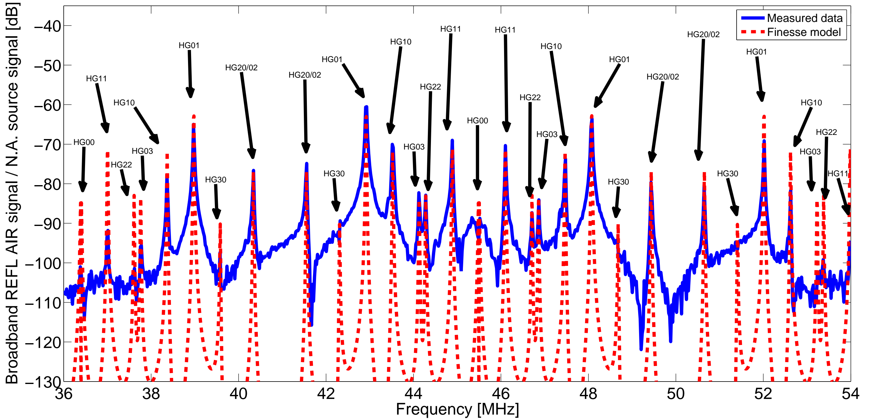
RF sideband sweep of H1 IMC 2013.10.04
