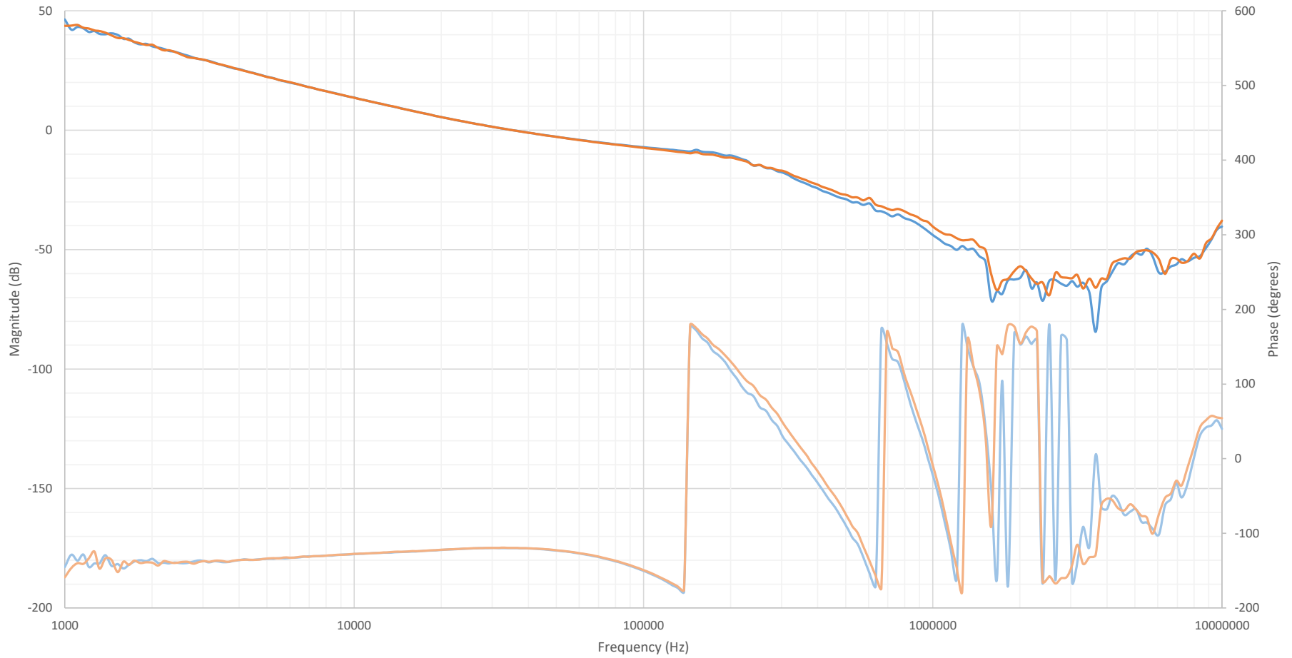
IMC FSS Common Gain Test 11-13-2024
