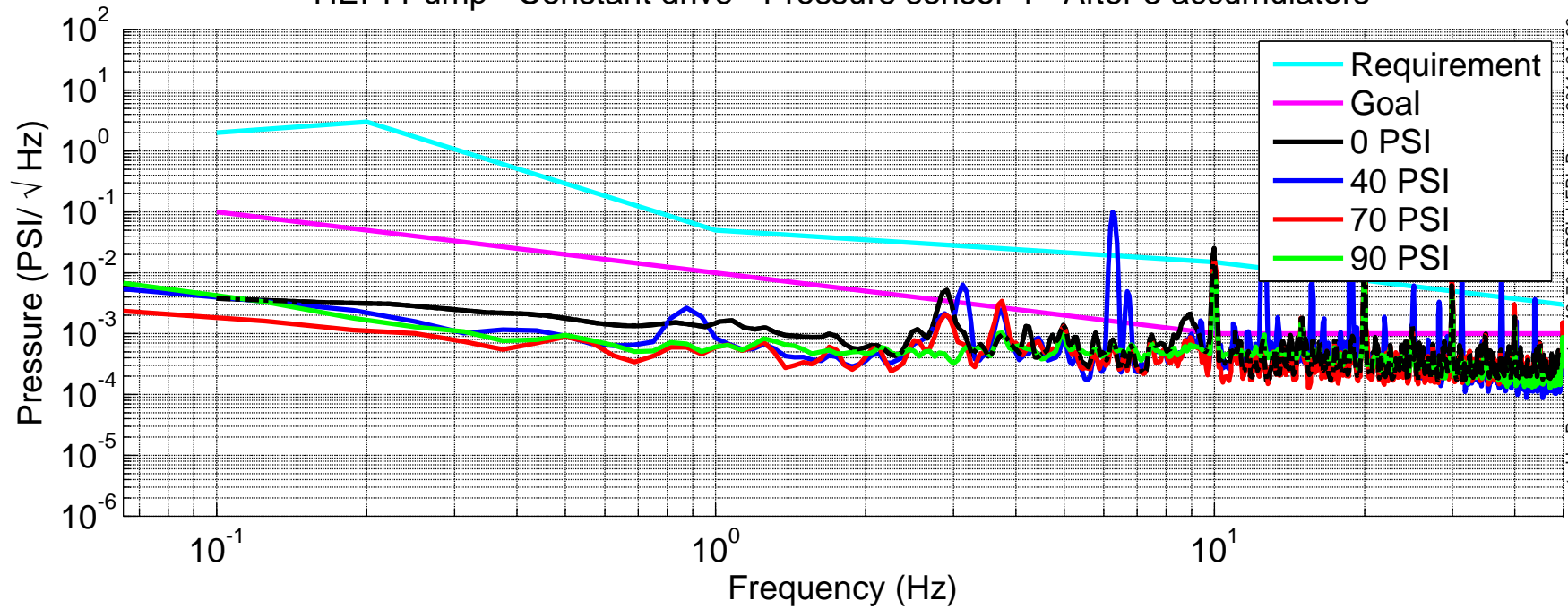
HEPI Pump - Constant drive - Pressure sensor 4 - After 3 accumulators
