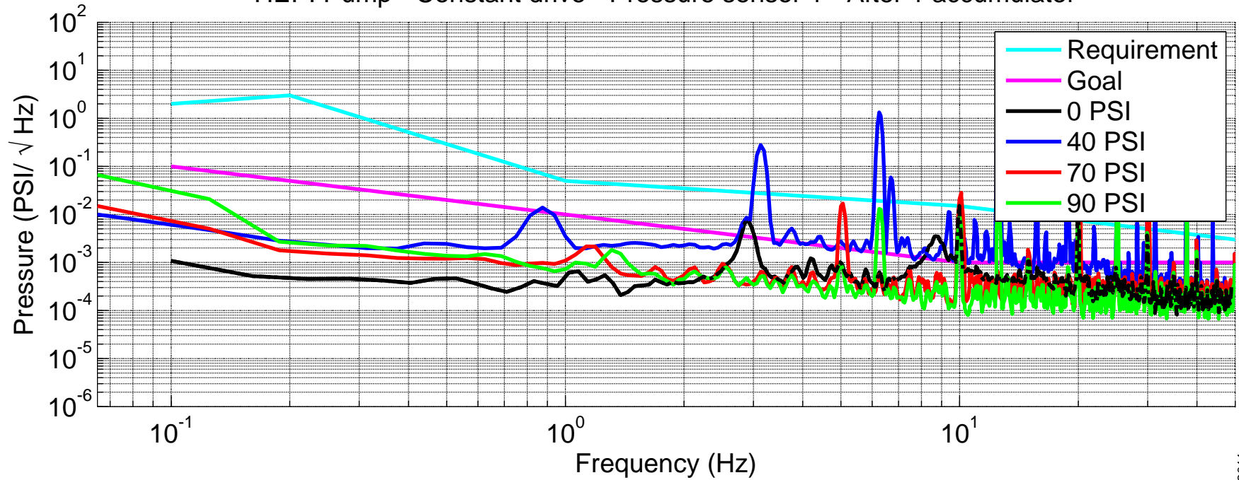
HEPI Pump - Constant drive - Pressure sensor 1 - After 1 accumulator
