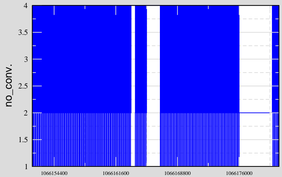
Ch 3: H0:PEM-CS_DUST_LAB2_STATE
