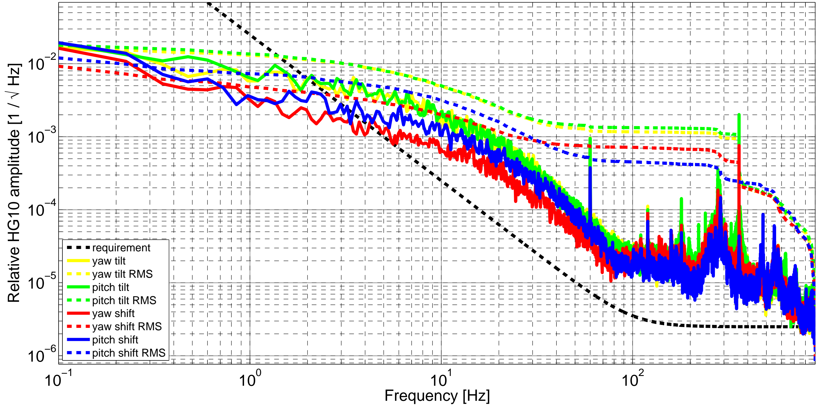
IMC input beam jitter (measured from RIN at IM4 trans)
