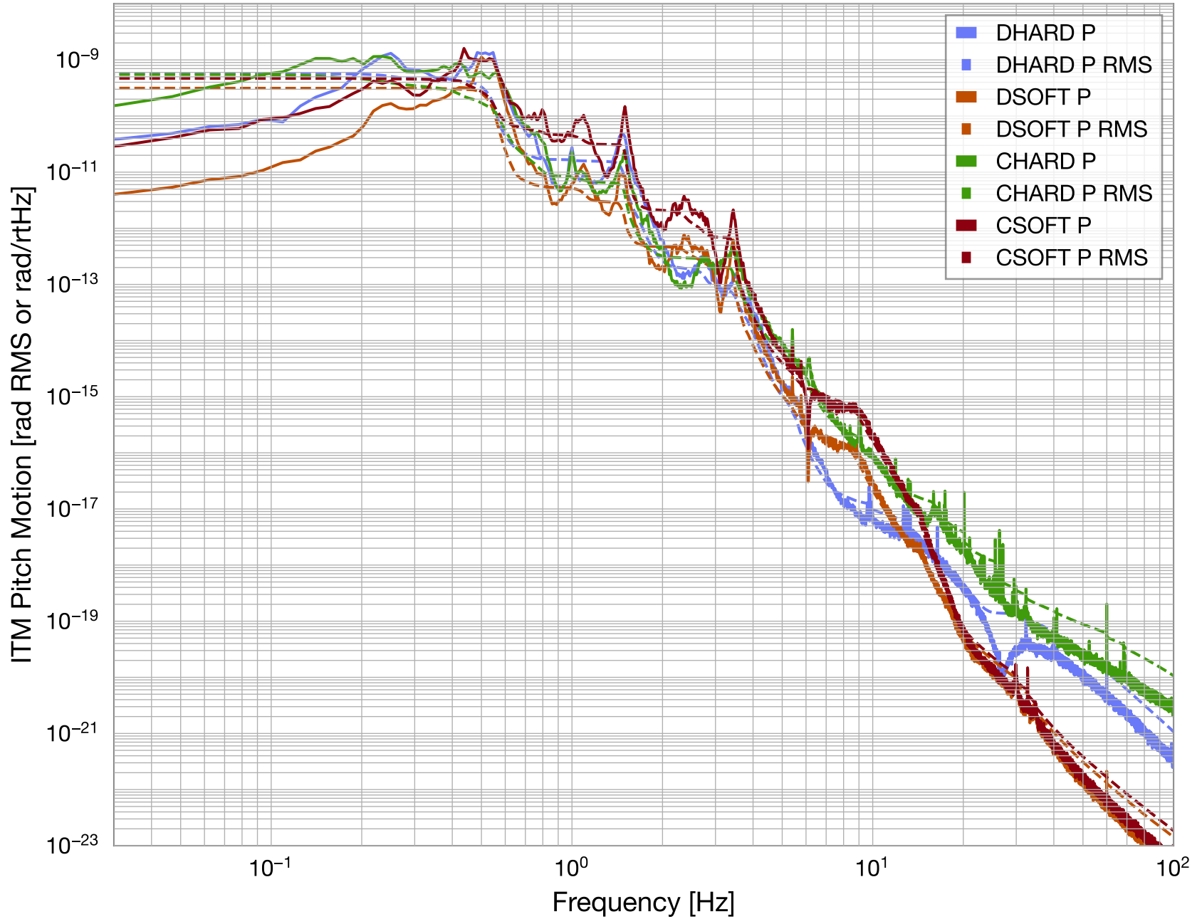
Test Mass Motion from ASC Drive
