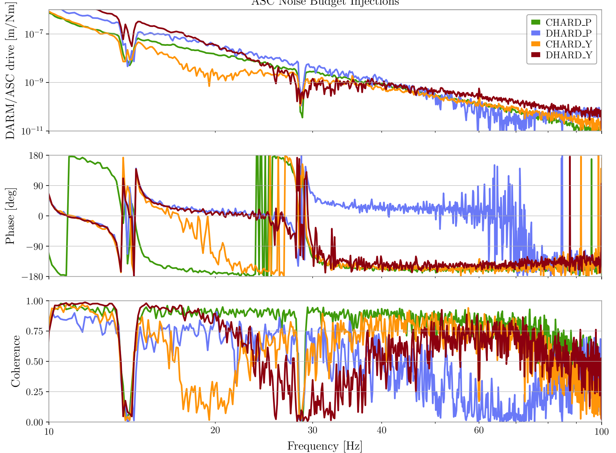
ASC Noise Budget Injections
