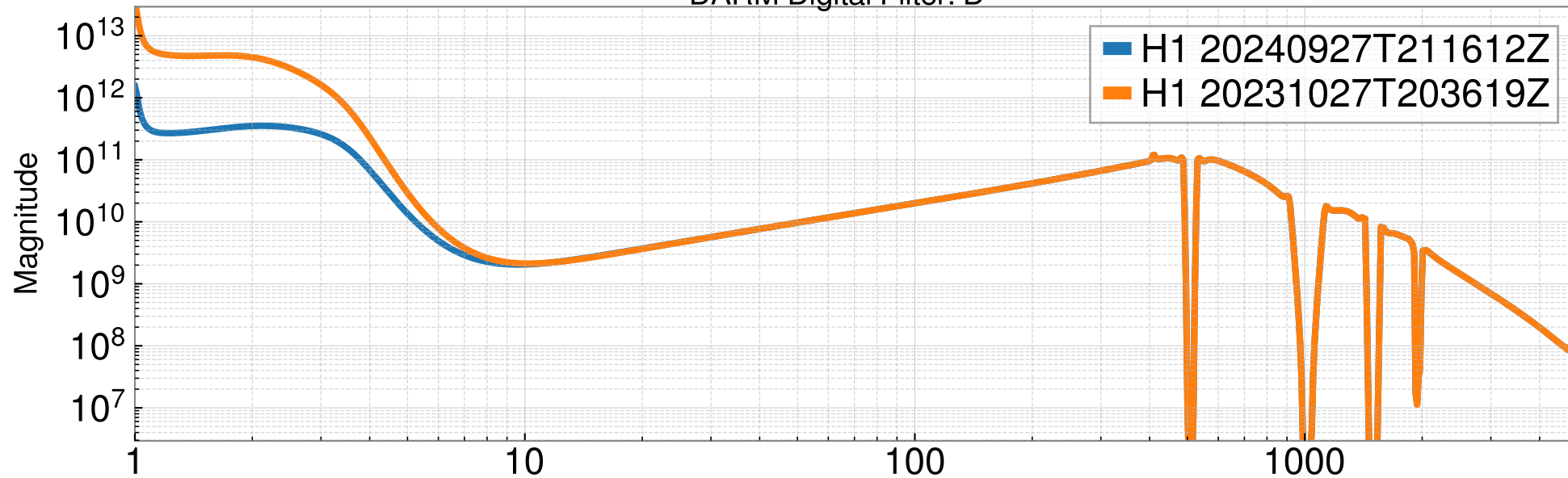
DARM Digital Filter: D
