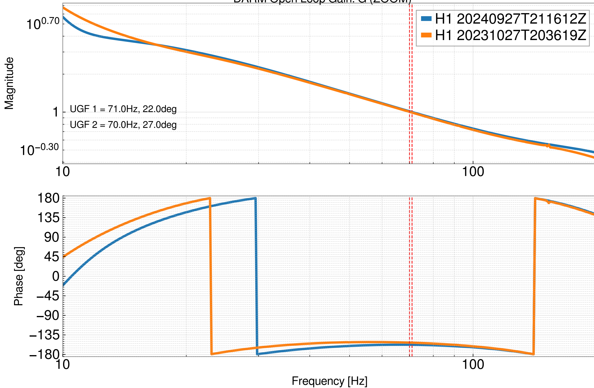
DARM Open Loop Gain: G (ZOOM)
