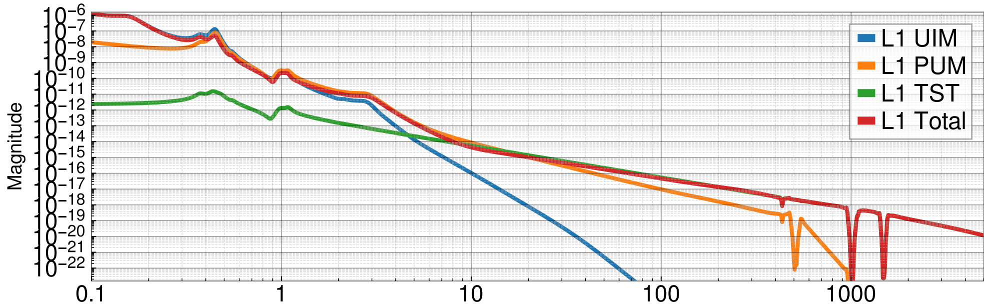
Act. stage LOCK_IN to Displ.
