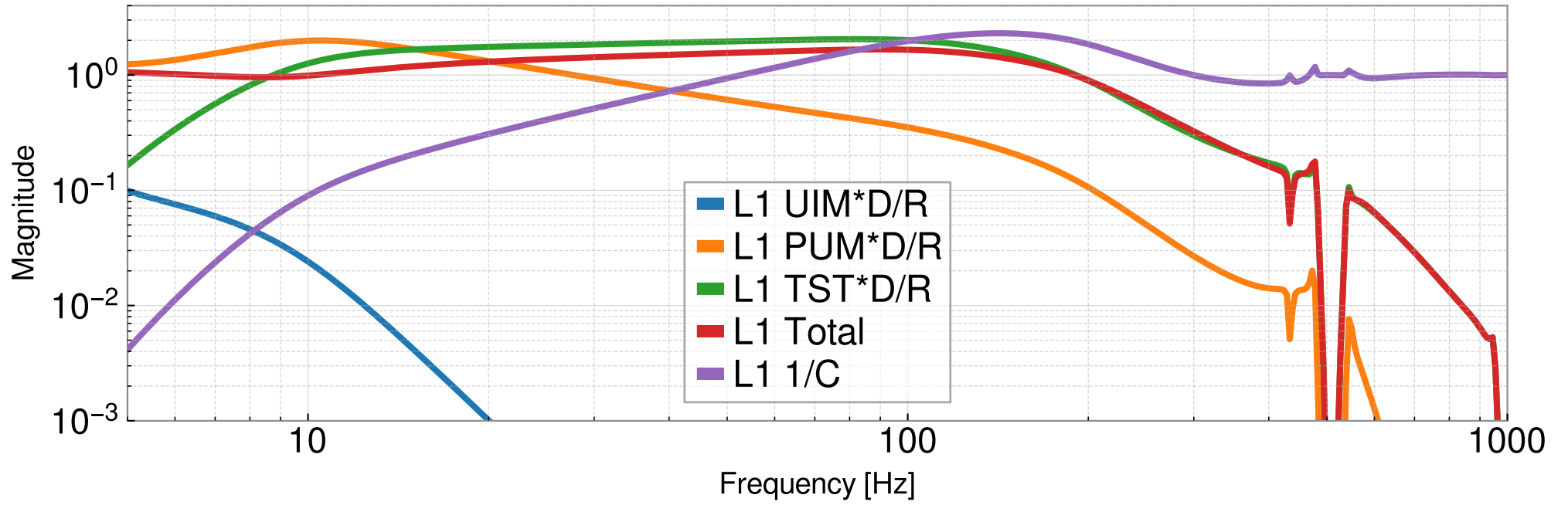
Act. stage relative contributions
