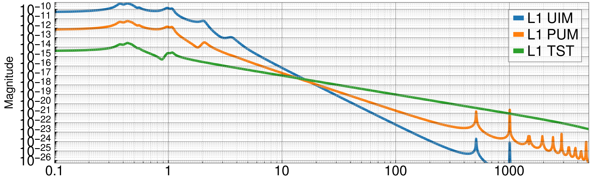
Act. stage strength
