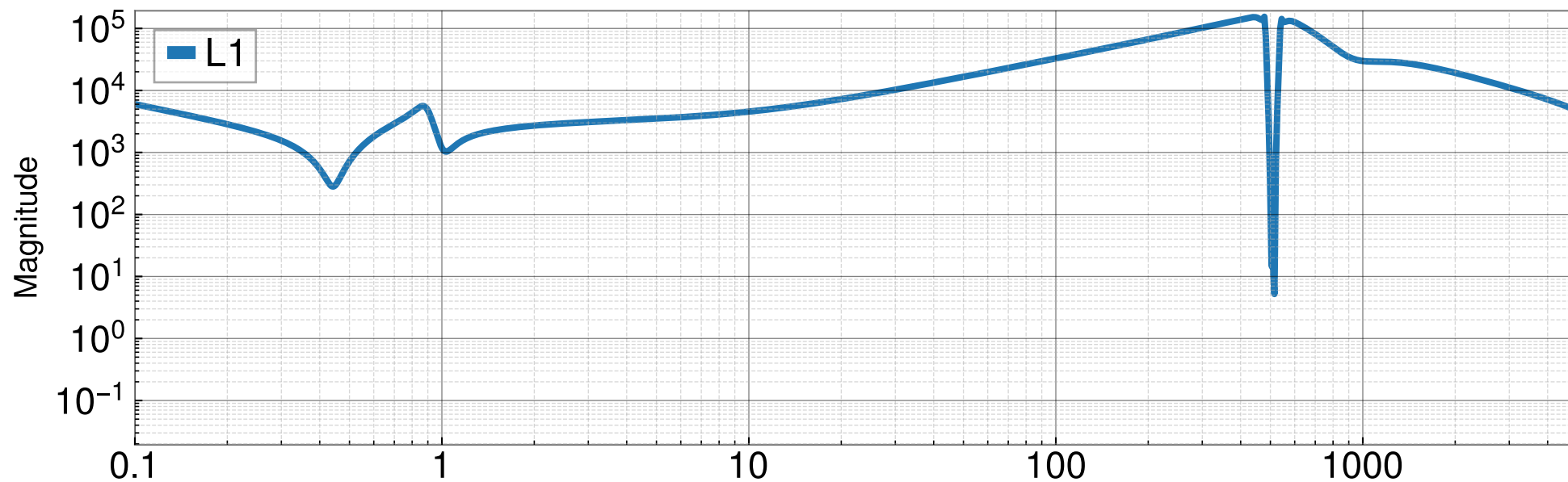
DARM Digital Filter: D
