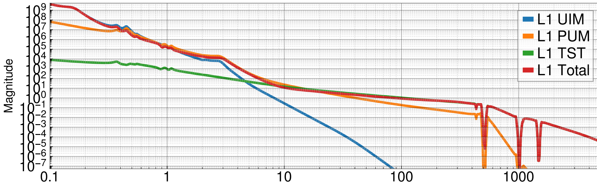
Act. stage DARM_IN to Disp. (D*A)
