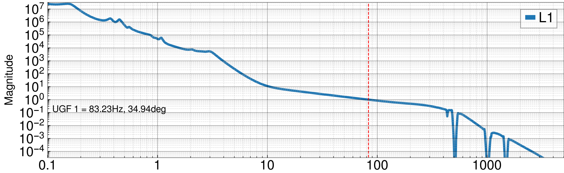
DARM Open Loop Gain: G
