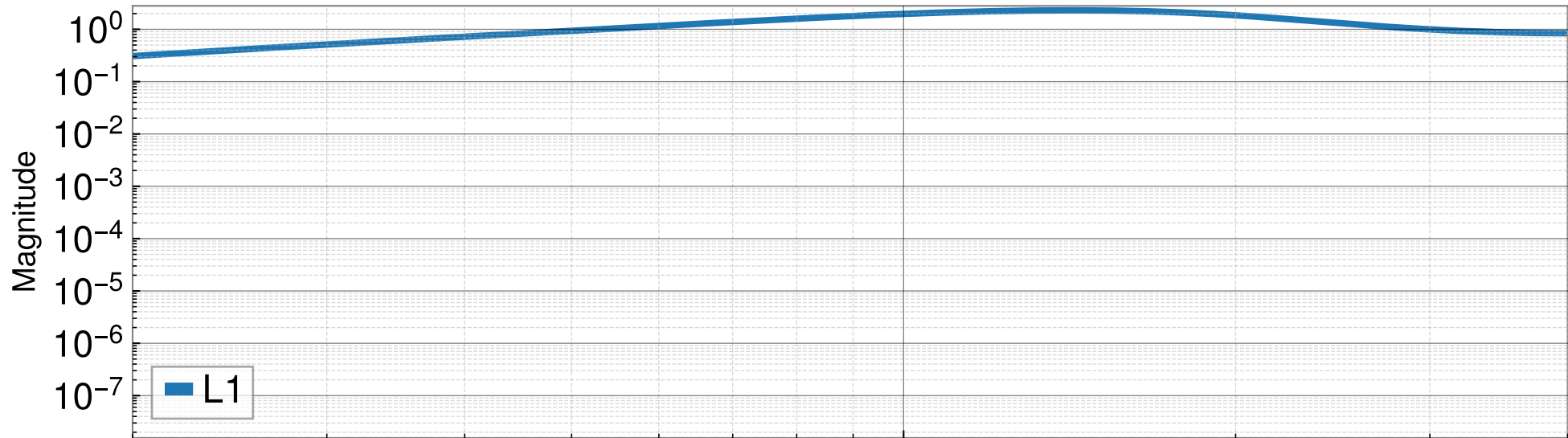
DARM Closed Loop Gain: 1/(1+G) (ZOOM)
