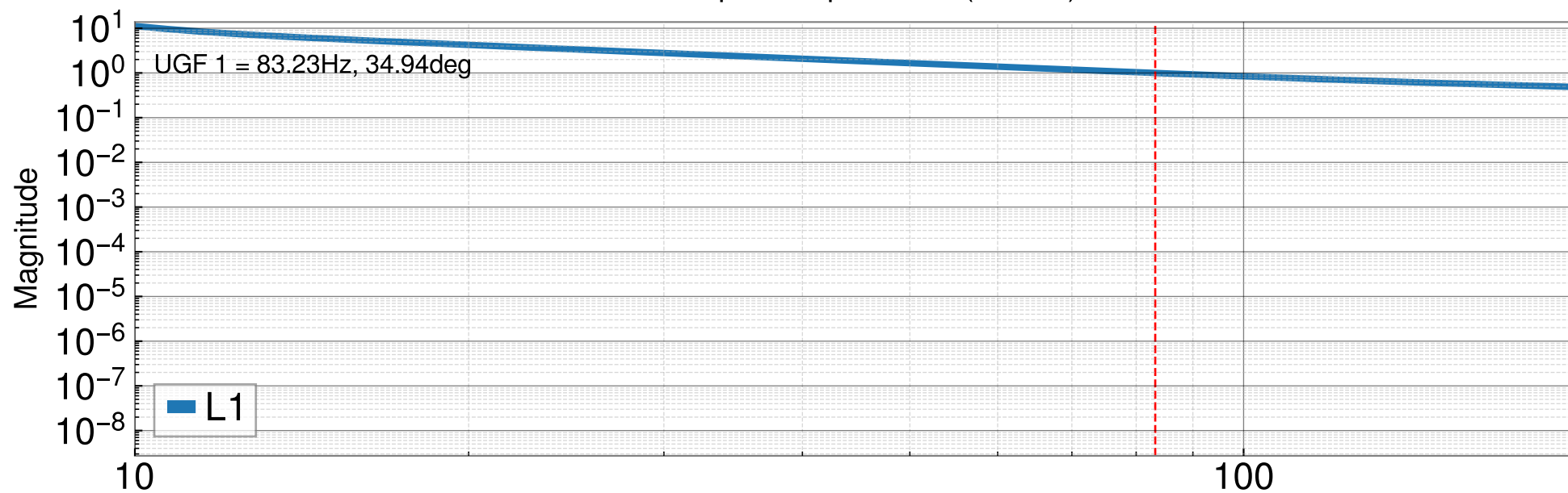
DARM Open Loop Gain: G (ZOOM)
