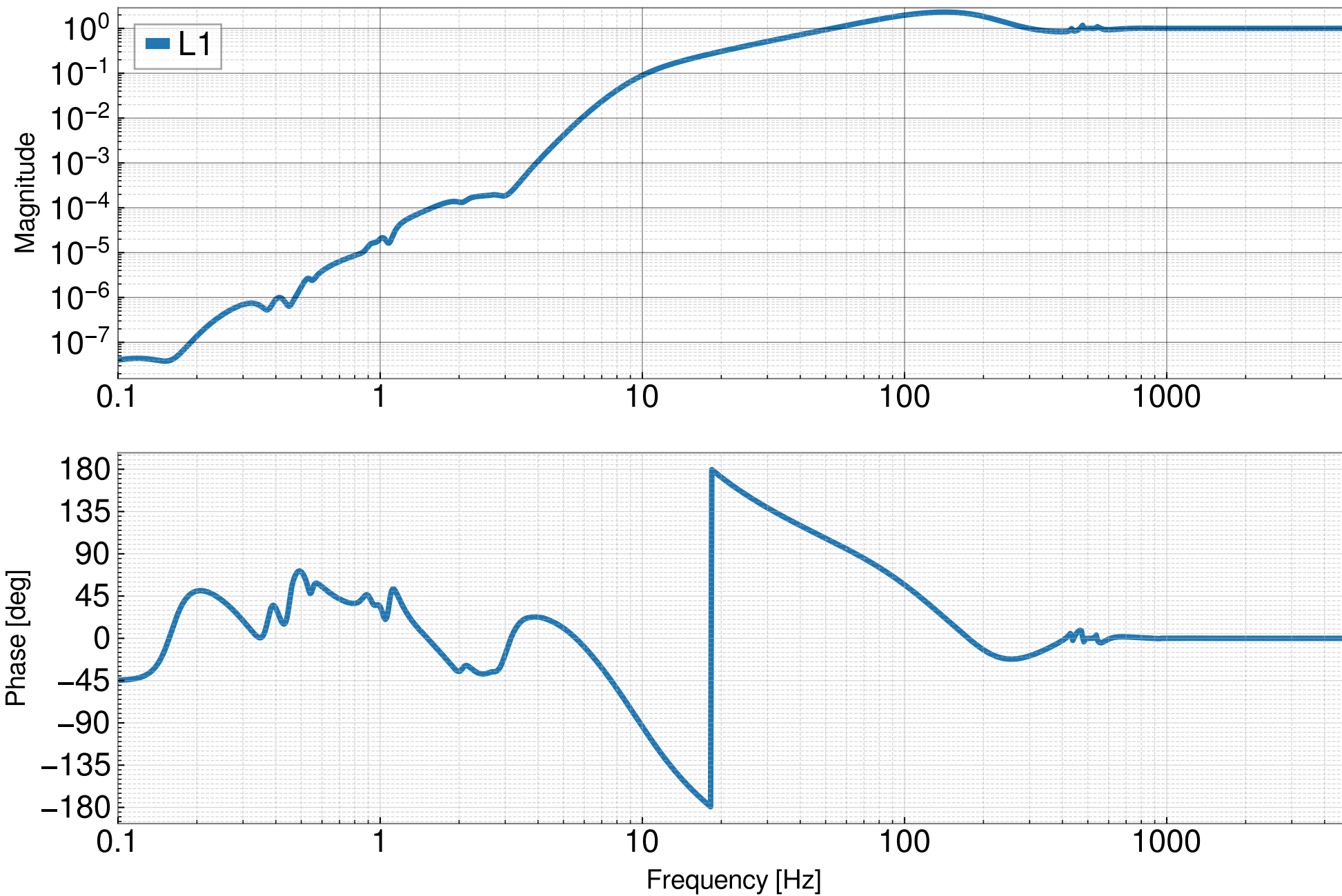
DARM Closed Loop Gain: 1/(1+G)
