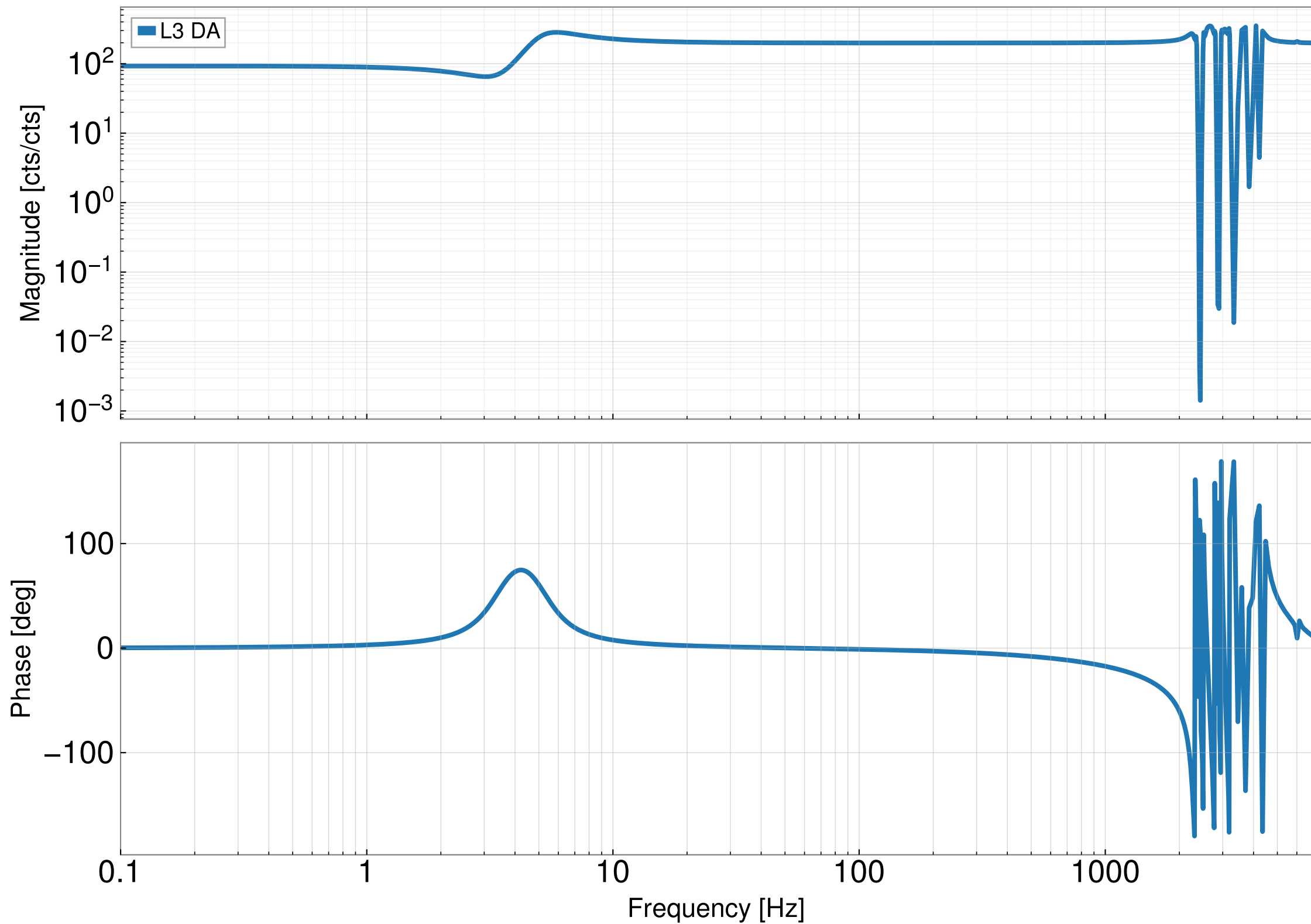
DARM-ctrl to L3 counts Measurement 2025-01-23 T21:11:18
