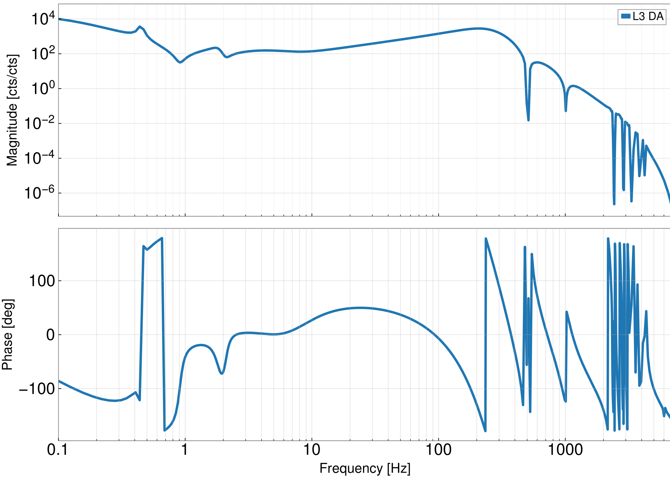
DARM-ctrl to L2 counts Measurement 2025-01-23 T21:11:18
