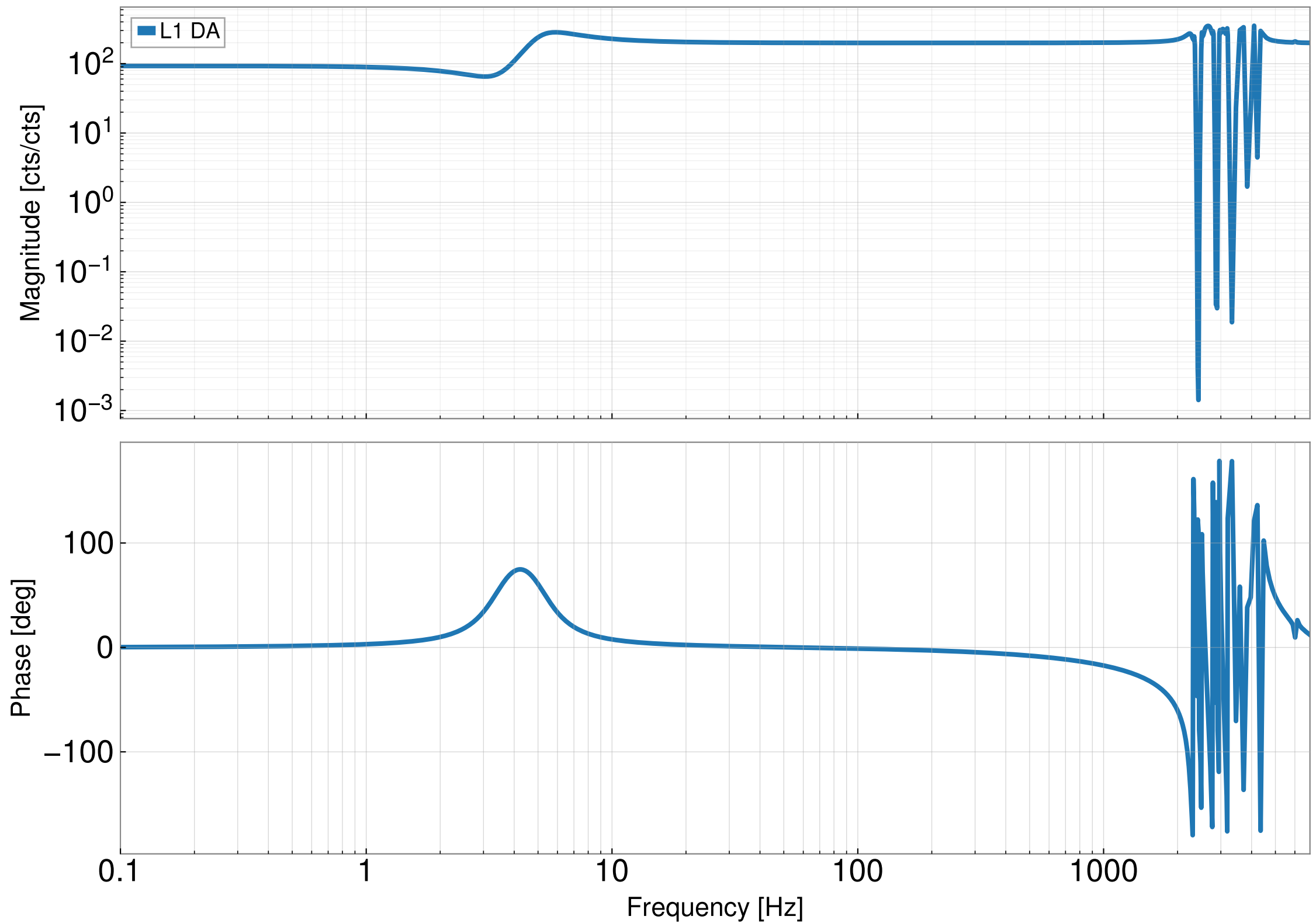
DARM-ctrl to L1 counts Measurement 2025-01-23 T21:11:18
